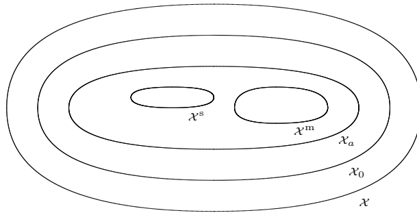
Fig. 2.2 Illustration of the structure of the sets \mathcal{X}_a 's (see definition (2.22)) with 0 < a < V^m .
