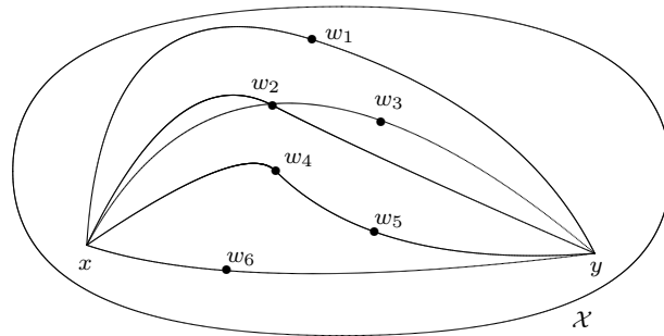
Fig. 2.3 Illustration of the notion of gate between two configurations x and y . The case depicted here is the following: \mathcal{S}(x, y) = \{w_1, \dots, w_6\} . The optimal paths in \Omega_{x,y}^{\text{opt}} are represented by the five black lines. The minimal gates are \{w_1, w_2, w_4, w_6\} and \{w_1, w_2, w_5, w_6\} . Any other subset of \mathcal{S}(x, y) obtained by adding some of the missing saddles to one of the two minimal gates is a gate.
