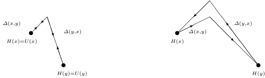
Fig. 2.1 Illustration of the result in Corollary 2.1. The picture on the left refers to the weak reversible case, whereas the picture on the right refers to the general dynamics with rare transitions.
