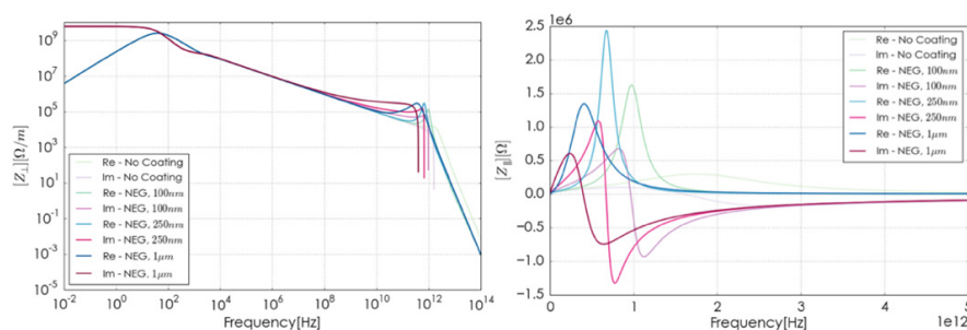
Figure 1: Real and imaginary part of the transverse (left) and longitudinal (right) RW impedances as a function of the frequency in the case of no coating and NEG coating with different thicknesses.
