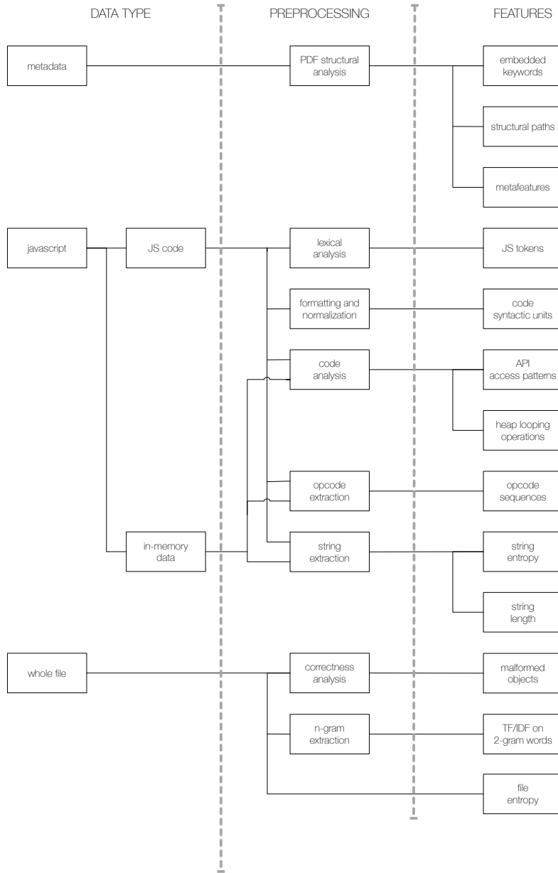
Figure 2: Taxonomy of features used in literature for PDF malware detection.
