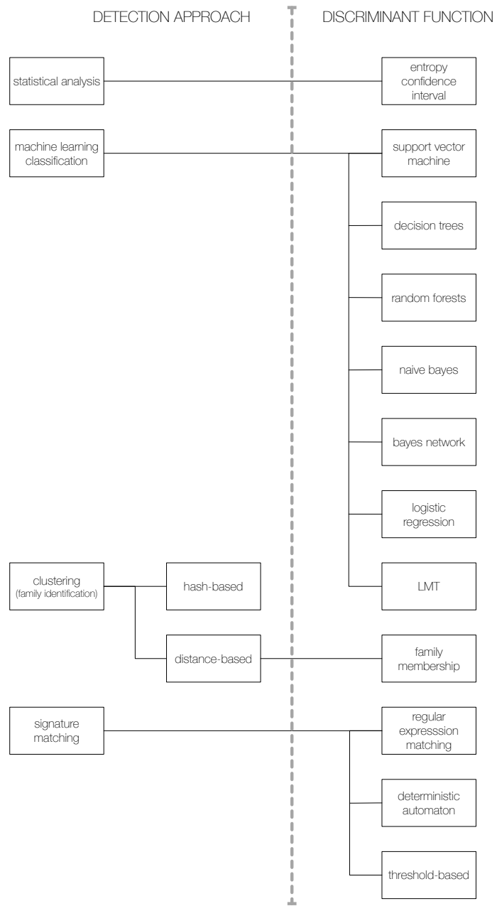
Figure 3: Taxonomy of approaches used in literature for PDF malware detection.
