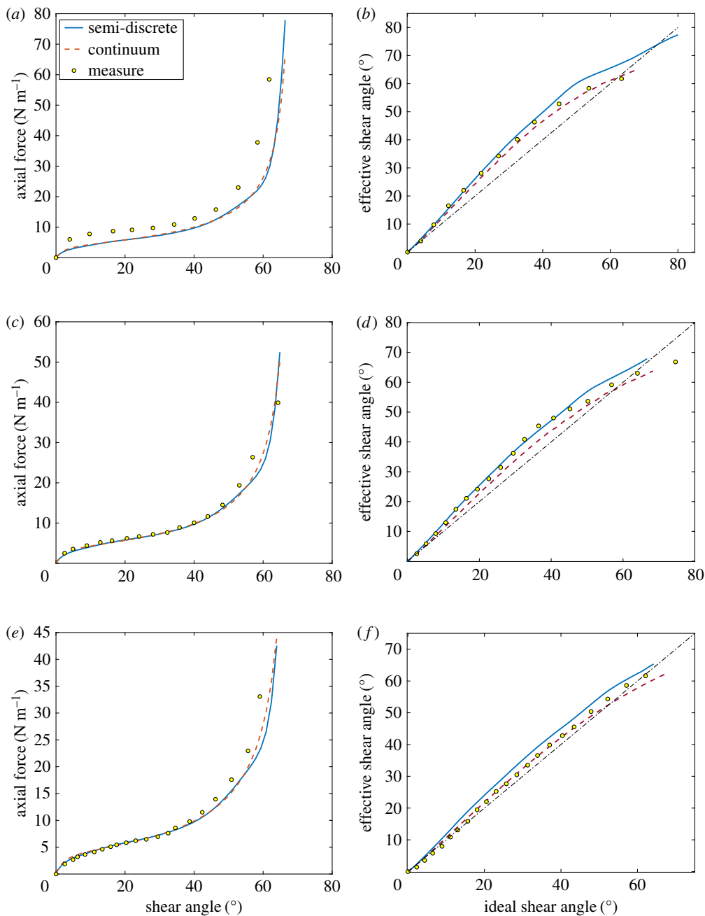
Figure 4. UBE test for the samples of size: (a,b) 100 × 200 mm; (c,d) 150 × 300 mm; (e,f) 200 × 400 mm. (a,c,e) Normalized axial force versus shear angle. (b,d,f) Effective shear angle versus ideal shear angle. (Online version in colour.)
