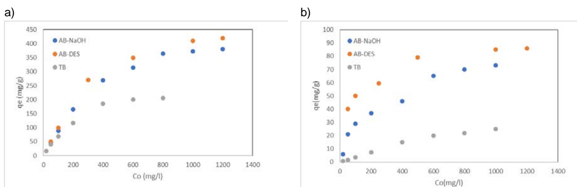
Figure 1: Adsorption capacities as a function of the initial dye concentration of the three biochars a) with methylene blue solutions; b) with rhodamine b solutions.
