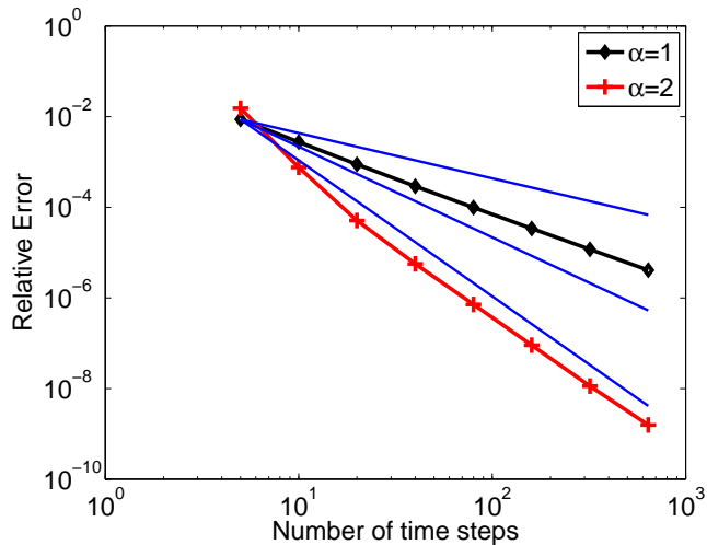
Figure 2: Error with respect to the number of steps for g in (99). The straight lines indicate slopes 1, 2 and 3, respectively.
