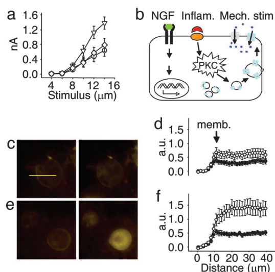
Fig. 5. PKC activation up-regulates MA currents by a mechanism involving insertion of new channels into the membrane. (a) TeNT inhibits sensitization of MA currents by PMA. Shown are average responses to increasing mechanical stimulation (up to 14 \mu m) in neonatal neurons. PMA alone up-regulates MA currents ( \nabla ; peak: 1.38 \pm 0.16 nA, n = 24 ; P < 0.005 vs. control), but after an 8-h incubation in TeNT (20 nM), PMA had no effect on current amplitude ( \cap ; mean at 14 \mu m: 0.79 \pm 0.18 nA, n = 24 ; P < 0.05 vs. PMA-treated cells). Peak control current was 0.64 \pm 0.16 nA ( \circ , n = 16 ). (b) Schematic representation of the proposed mechanisms underlying peripheral sensitization to mechanical stimulation. NGF, acting via trkA receptors, increases transcription of MA channels, which are packaged into vesicles. Activation of PKC by proinflammatory signals induces fusion of the vesicles and insertion of new mechanosensitive channels into the cell membrane. (c) Epifluorescence images taken 5 min (Left) and 20 min (Right) after FM1-43, a marker of vesicle recycling, was applied to neurons bathed in control extracellular solution (horizontal bar: 40 \mu m.) (d) Quantitative analysis of the mean fluorescence (arbitrary units) in 11 neurons whose images were taken as described in c ( \bullet , 5 min; \circ , 20 min), measured along a 40- \mu m segment (indicated by yellow line in c). Segments were drawn such that each cell's profile could be superimposed for comparison. (e) As in c, but FM1-43 was coapplied with 30 nM PMA. (f) Analysis as in d, but neurons ( n = 12 ) were treated with PMA as in e.
