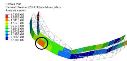
Fig. 11. Example of shell stress trend with the maximum stressed zone in the black circle.
