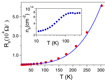
FIG. 6. Sheet resistance R (dots) of the q-2DES under amorphous LAO, measured on sample B and fit (solid line) to the large-polaron model of Eq. (8). Inset: surface charge density n_s vs temperature as determined by Hall measurements.
