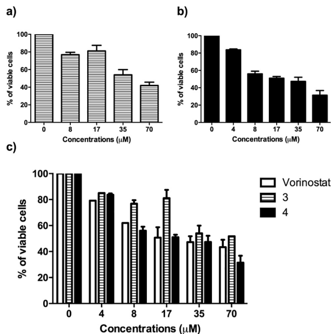
Fig. 3. Cell viability after 24 h treatment of MCF-7 cells with a) compound 3 , b) compound 4 and c) compounds 3 and 4 in comparison with Vorinostat.
