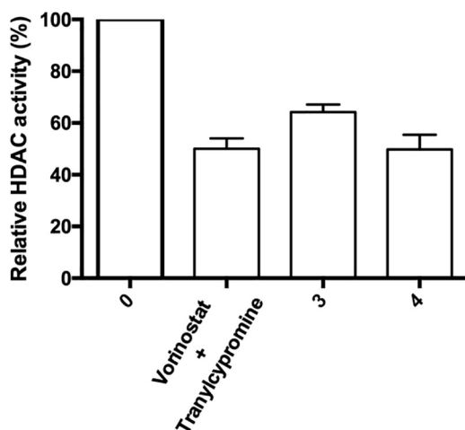
Fig. 4. Relative HDAC activity of Vorinostat (35 \mu\text{M} ) plus Tranylcypromine (1000 \mu\text{M} ), compounds 3 (70 \mu\text{M} ) and 4 (17 \mu\text{M} ) on MCF-7 nuclear extracts.
