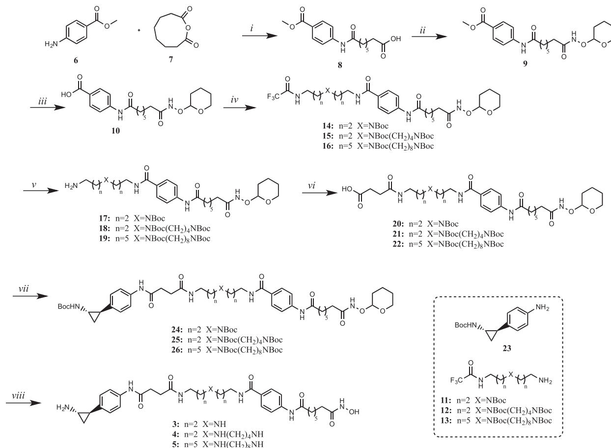
Scheme 1. i) THF, rt, 12 h; ii) NH 2 OTHP, EDC, DMAP, Et 3 N, DCM, rt, 12 h; iii) NaOH, MeOH, 50 °C, 2 h; iv) 11–13 , EDC, HOBt, Et 3 N, THF, rt, 16 h; v) NaOH, MeOH, rt, 16 h; vi) succinic anhydride, Et 3 N, DCM, rt, 16 h; vii) 23 , EDC, DMAP, DCM, rt, 24 h; viii) HCl 4 M/dioxane, DCM, rt, 12 h.
