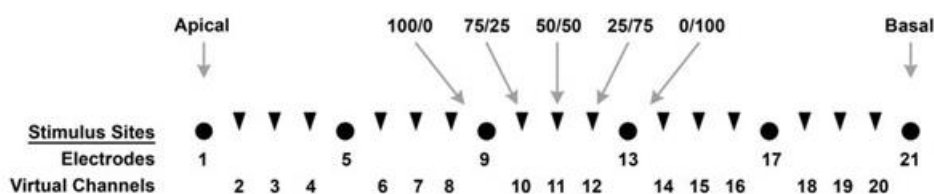
Figure 6. Diagram of stimulus sites used in virtual channel interleaved sampling processors and other similar processors.
