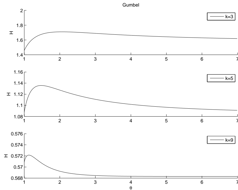
Figure A2. Plot of the dependence of the entropy function H on the parameter \theta . The same comments as for Figure 6 hold.
