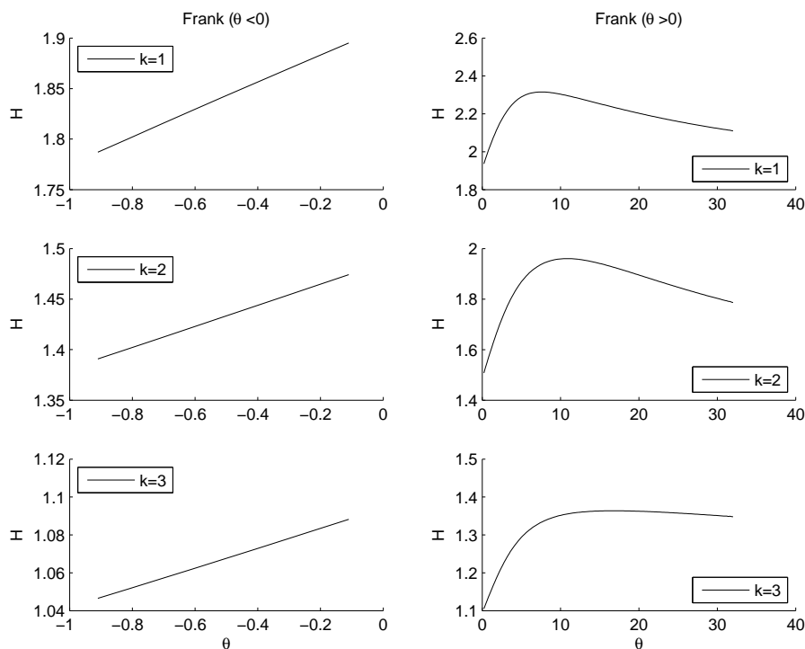
Figure A3. Plot of the dependence of the entropy function H on the power law exponent k . The same comments as for Figure 7 hold.
