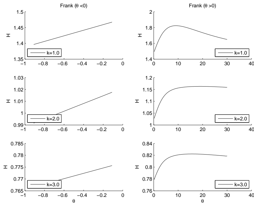
Figure A7. Plot of the dependence of the entropy function H on the parameter \theta . The same comments as for Figures 7 and A3 hold.
