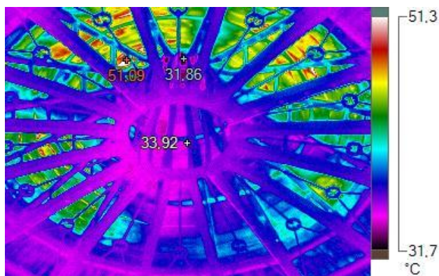
Figure 12. Thermal images of the dome
