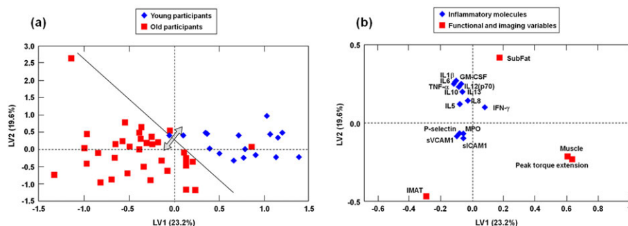
Figure 2 Scores (a) and loadings (b) plots showing the relationships among inflammatory, functional, and thigh composition parameters in the space spanned by the two latent variables (LV1 and LV2), as determined by multi-block PLS-DA. In the scores plot, the diagonal line and the double-headed arrow (added to facilitate interpretation) indicate the boundary between age groups and the direction along which the separation occurs, respectively. The loadings plot shows a negative correlation between subcutaneous fat (SubFat) and intermuscular adipose tissue (IMAT) volumes, and a positive correlation between IMAT volume and circulating levels of P-selectin, MPO, sVCAM-1, and sICAM-1.
