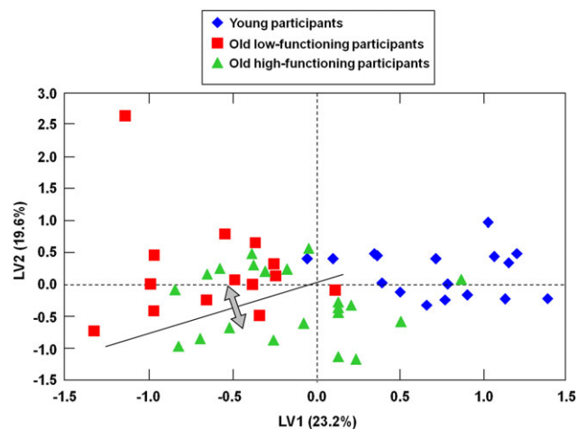
Figure 3 Scores plot showing the separation of participants according to inflammatory, functional, and thigh composition parameters in the space spanned by the two latent variables (LV1 and LV2), as determined by multi-block PLS-DA. The diagonal line (added to facilitate interpretation) corresponds to the boundary between older adults with SPPB >8 ('high-functioning') and those with SPPB \leq 8 ('low-functioning'). The double-headed arrow indicates the direction along which the separation occurs.
