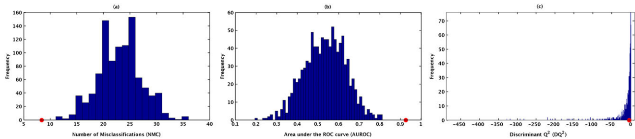
Figure 1 Distribution of (a) number of misclassifications (NMC), (b) area under the receiver operating characteristic (ROC) curve (AUROC), and (c) discriminant Q^2 ( DQ^2 ) values under their respective null hypothesis as estimated by permutation tests with 1000 randomisation (blue histograms) and the corresponding values obtained by the PLS-DA model on unpermuted data (red circles).
