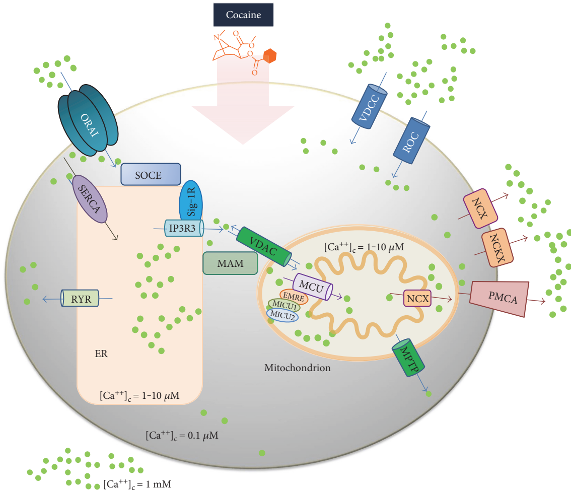
FIGURE 1: Main players of the cell \text{Ca}^{2+} molecular machinery as putative cocaine targets. Ideal intracellular \text{Ca}^{2+} concentration is maintained through complex equilibria among the extracellular space (1 mM), the cytoplasm (0.1 \mu\text{M} ), and the cellular stores (1.0–10 \mu\text{M} ), such as the mitochondrion, the endoplasmic reticulum (ER), the Golgi apparatus, and nucleus. The ion trafficking occurs via a variety of selective membrane channels, \text{Ca}^{2+} -binding proteins and transporters and ion exchangers and receptors, altogether responsible for \text{Ca}^{2+} import, export, and homeostasis. Import occurs at the level of (i) cell plasma membrane through the calcium release-activated \text{Ca}^{2+} channel protein 1 (ORAI1), the store-operated calcium entry channels (SOCE), and specific receptor-operated channels (ROC) such as AMPA, NMDA, TRPC, and the voltage-dependent calcium channels (VDCC); (ii) endoplasmic reticulum (ER) through the sarco/endoplasmic reticulum calcium ATPase (SERCA); (iii) mitochondria intermembrane space through the voltage-dependent anion channel (VDAC); and (v) in the matrix by the mitochondrial uniporter (MCU), in synergy with the mitochondrial calcium uptake (MICU) system. Extrusion occurs at the level of (i) cell plasma membrane mainly by the plasma membrane calcium ATPase (PMCA) and the sodium calcium exchangers (NCX) also potassium-dependent (NCKX) and (ii) the ER by the ryanodine (RYR) and the inositol 1,4,5-trisphosphate receptors (I P3R), as well as by the mitochondrial permeability transition pore (MPTP).
