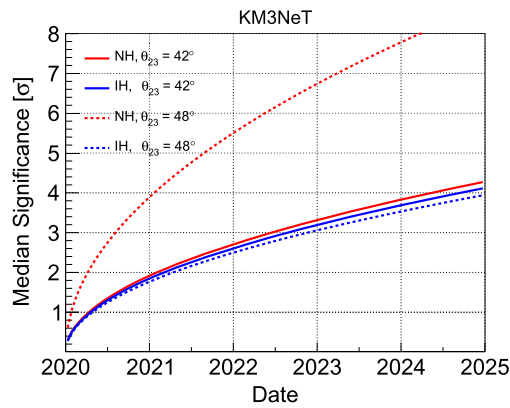
Figure 2. Median significance as a function of time for the determination of the neutrino mass hierarchy. The different lines denote expectations for different combinations of hierarchy and atmospheric mixing angle \theta_{23} . Note that the CP-violating phase \delta_{CP} has been assumed to be zero.
