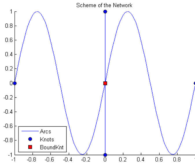
Figure 3.2: Test 1, structure of the graph.
