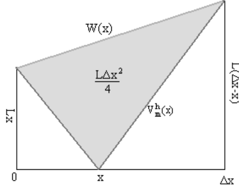
Figure 4.1: Bound on the L^1 error on a regular interval.
