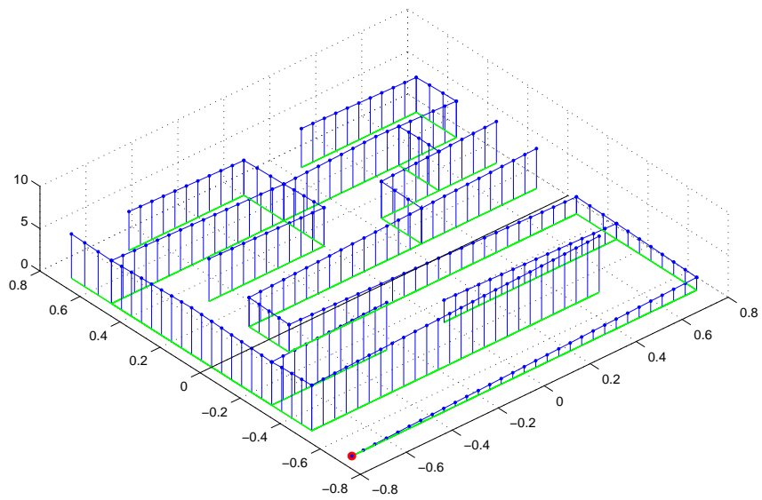
Figure 5.15: The graph that modelizes the labyrinth.
