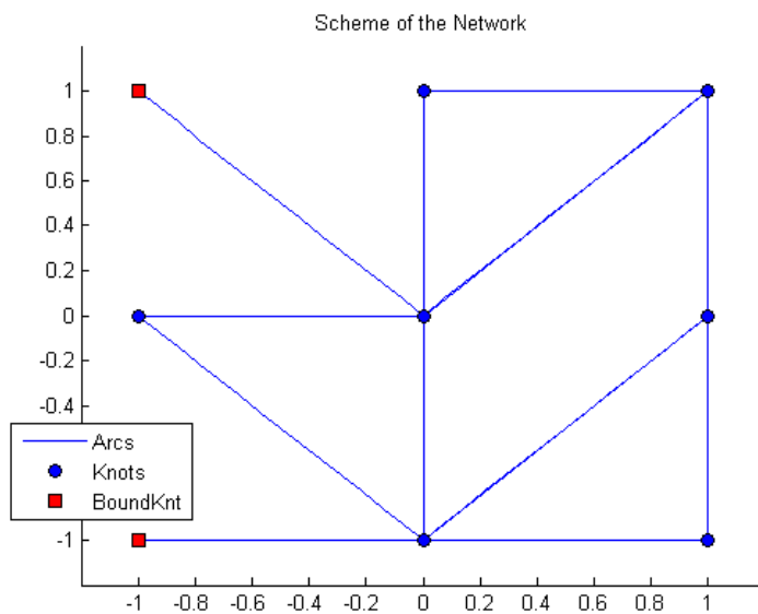
Figure 3.4: Test 2, structure of the graph.
