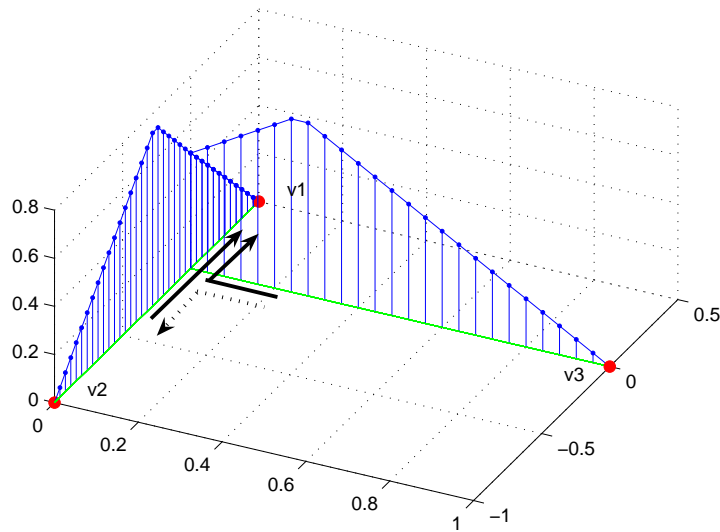
Figure 3.1: Remark 3.3, solid arrows, supersolution condition verified, dashed arrows supersolution condition not verified.
