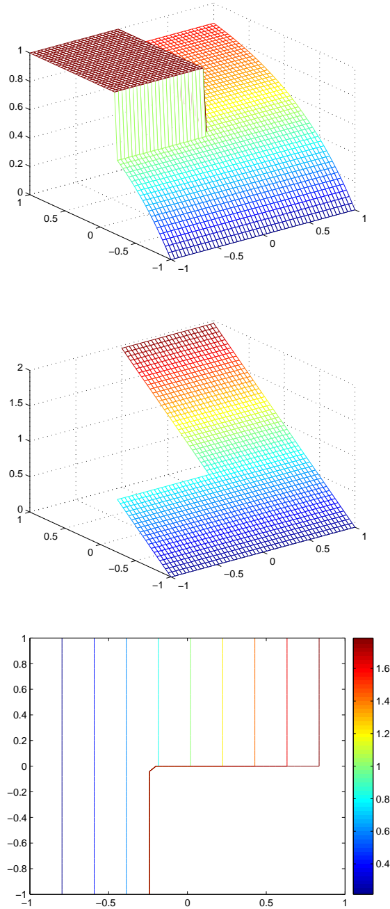
Figure 5.17: Function V (Kruscov transformed), U (mesh and level sets).
