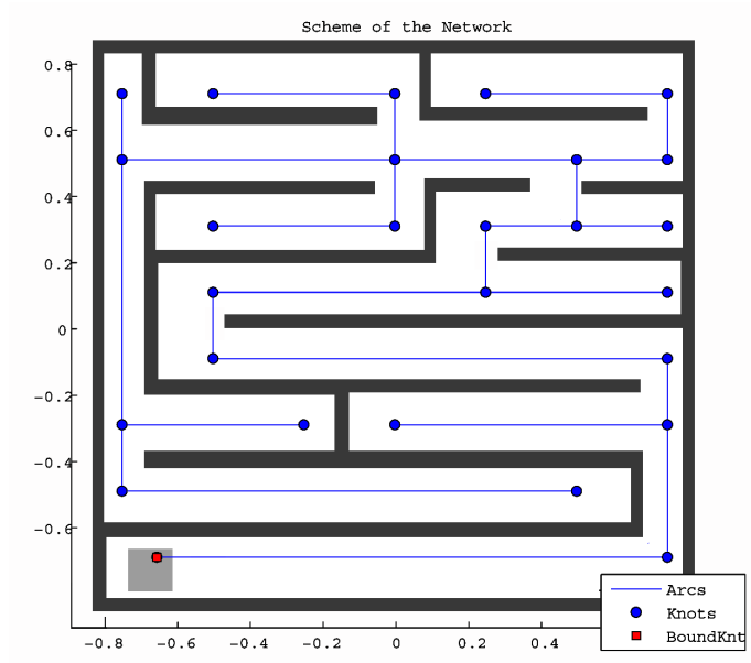
Figure 5.15: The graph that modelizes the labyrinth.
