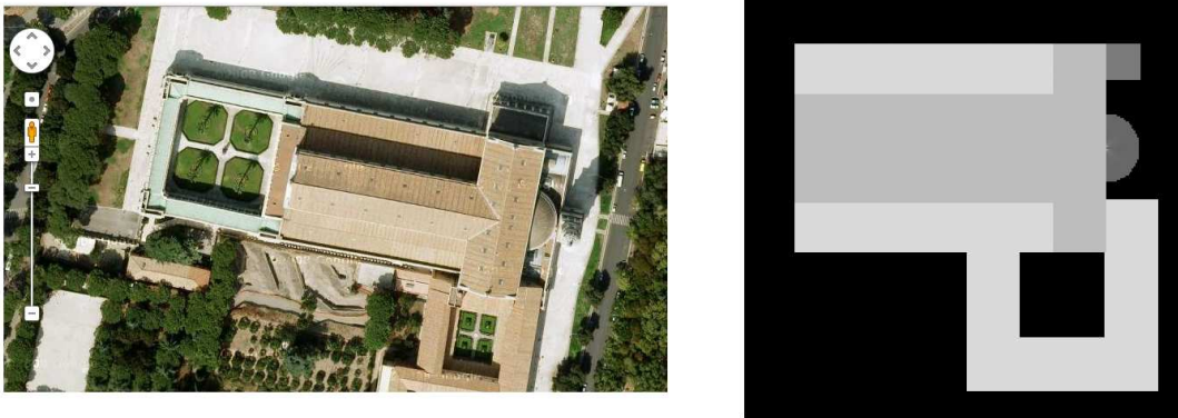
Figure 5.9: Basilica of Saint Paul Outside the Walls: satellite image and simplified sfs-datum.
