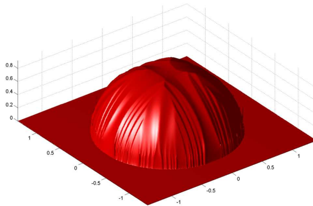
Figure 5.5: Half sphere: original shape and sfs-datum.
