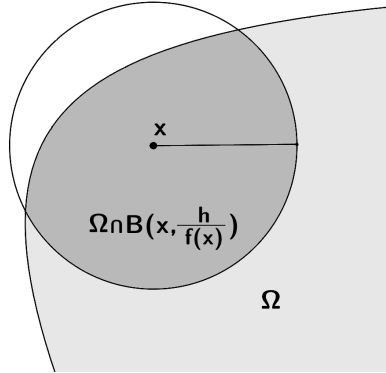
Figure 2.2: The set \Omega \cap B(x, \frac{h}{f(x)}) .
