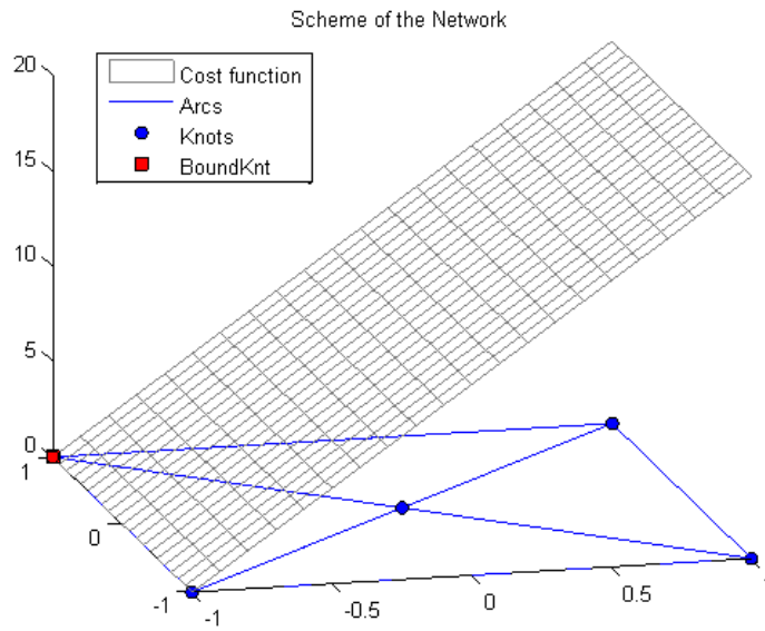
Figure 3.6: Test 3, structure of the graph.
