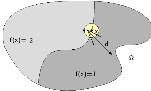
Figure 2.1: A simple condition where the sufficient condition is verified.
