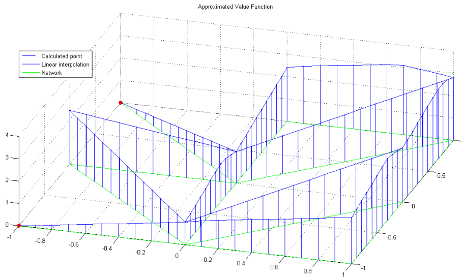
Figure 3.5: Test 2, \Delta x = 0.1 .
