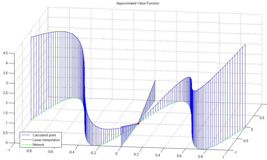
Figure 3.3: Test 1, \Delta x = 0.025 .
