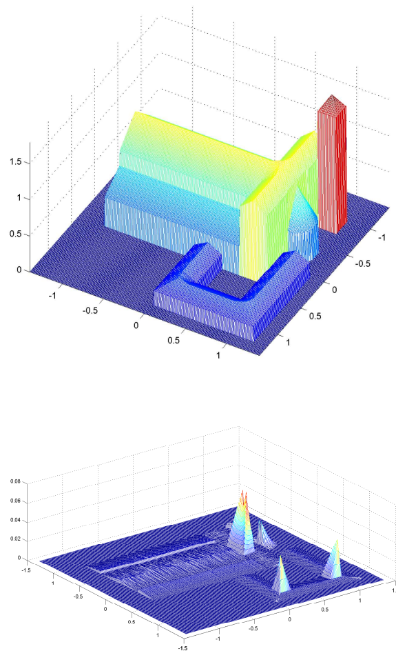
Figure 5.12: Basilica: reconstructed shape and modulus of the error.
