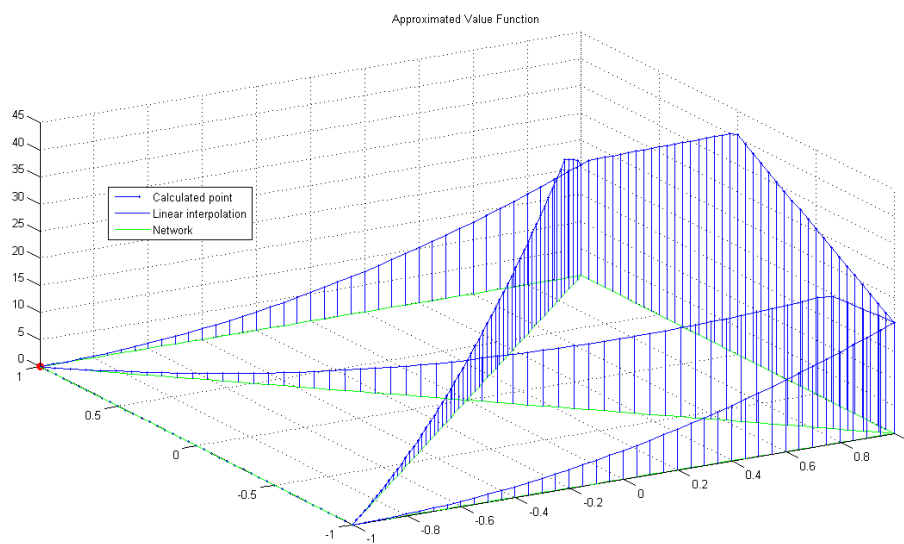
Figure 3.7: Test 3, \Delta x = 0.05 .
