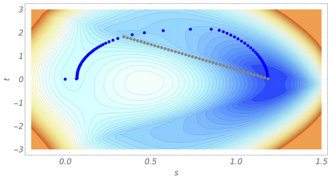
Figure 9. Total energy, \mathcal{U} , for d = 13 mm and \theta = 5^\circ . The blue points show a possible eversion path; the grey points indicate how the path is altered when contact is enforced between the deformed shell and the magnet.
