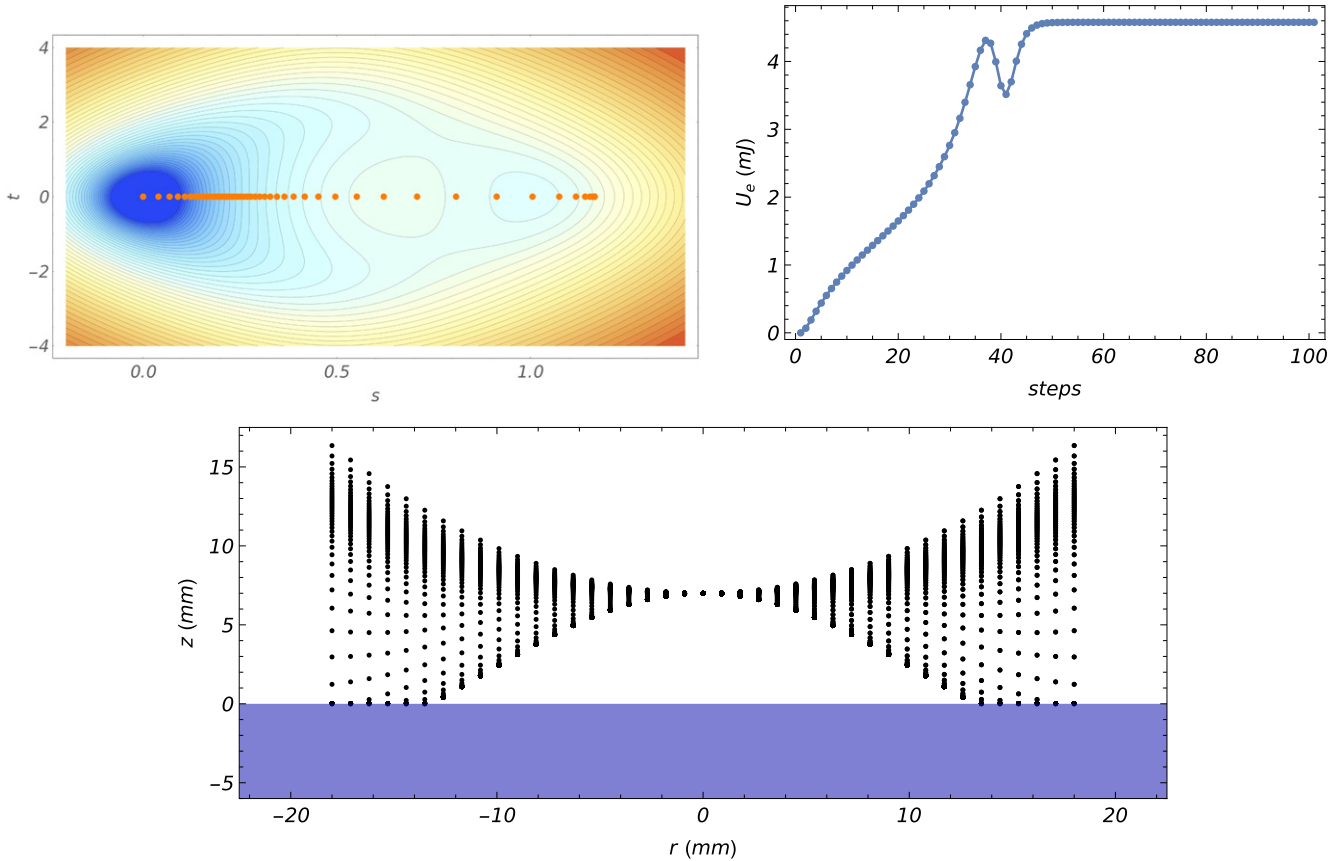
Figure 8. Top left: the eversion path in figure 7 superposed onto the landscape of elastic strain energy, \mathcal{U}_e . Top right: values of \mathcal{U}_e from (a) plotted with respect to fixed time intervals see the finite element data from figure 1. Bottom: the resulting axisymmetrical shell configurations during eversion.
