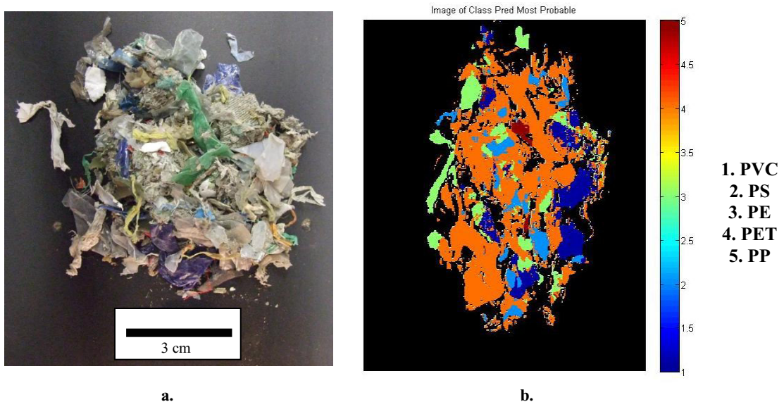
Fig. 2. SRF representative sample (a) and predicted image (b) as resulting from PLS-DA modelling.
