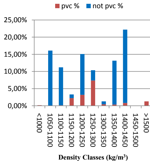
Fig. 1. Density distribution of the coarse product selected from the sink fraction resulting from laboratory sink-float separation of the heavy fraction as resulted from the industrial processing. The distribution of the PVC particles is displayed in red, are displayed in blue the particles which do not contain PVC.
