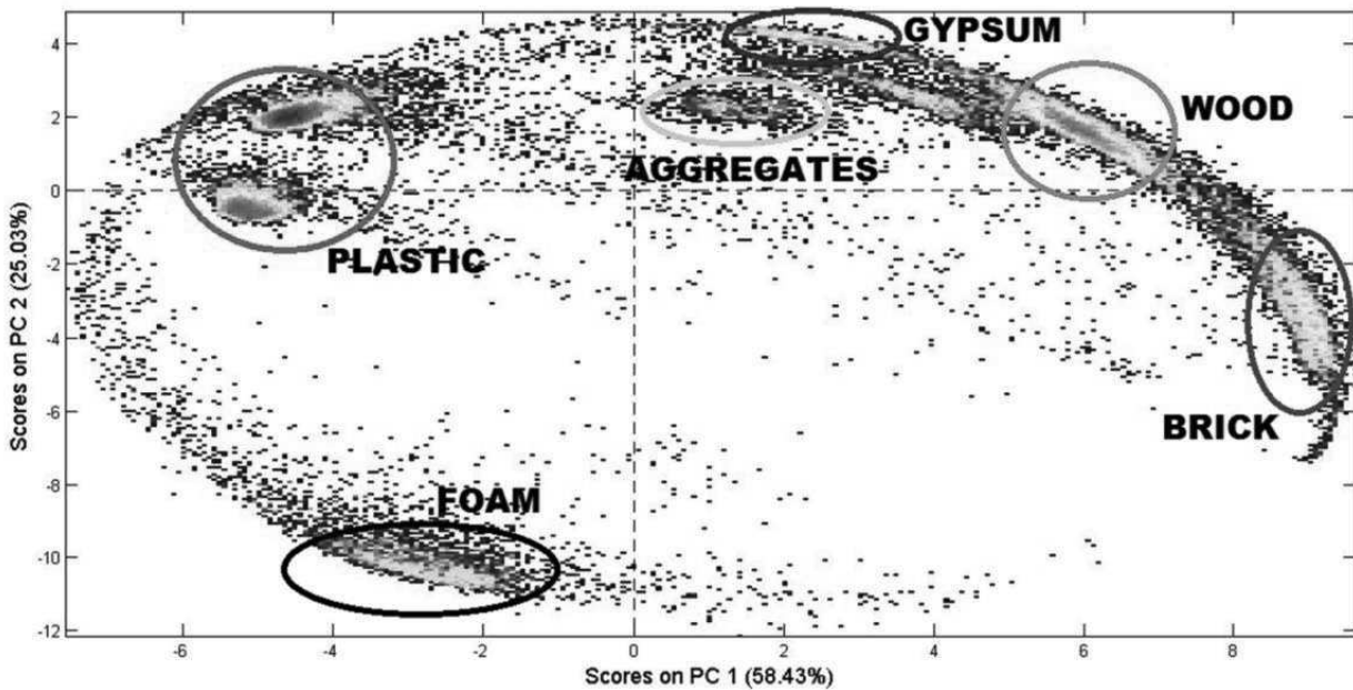
Figure 19: PCA score plot: Experimental set-up 1 pixels projection onto the space of PC1 vs PC2.
