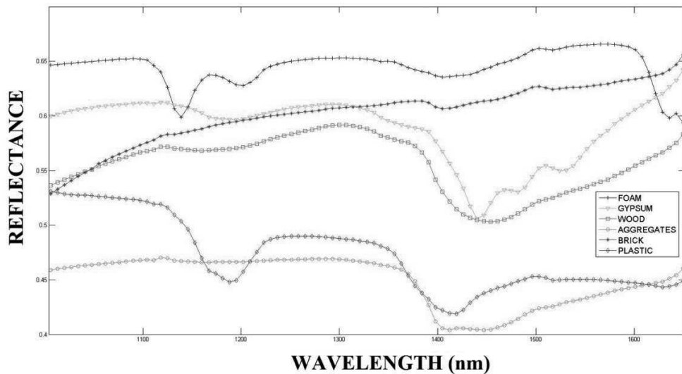
Figure 17: Acquired spectra of the six different analysed materials.
