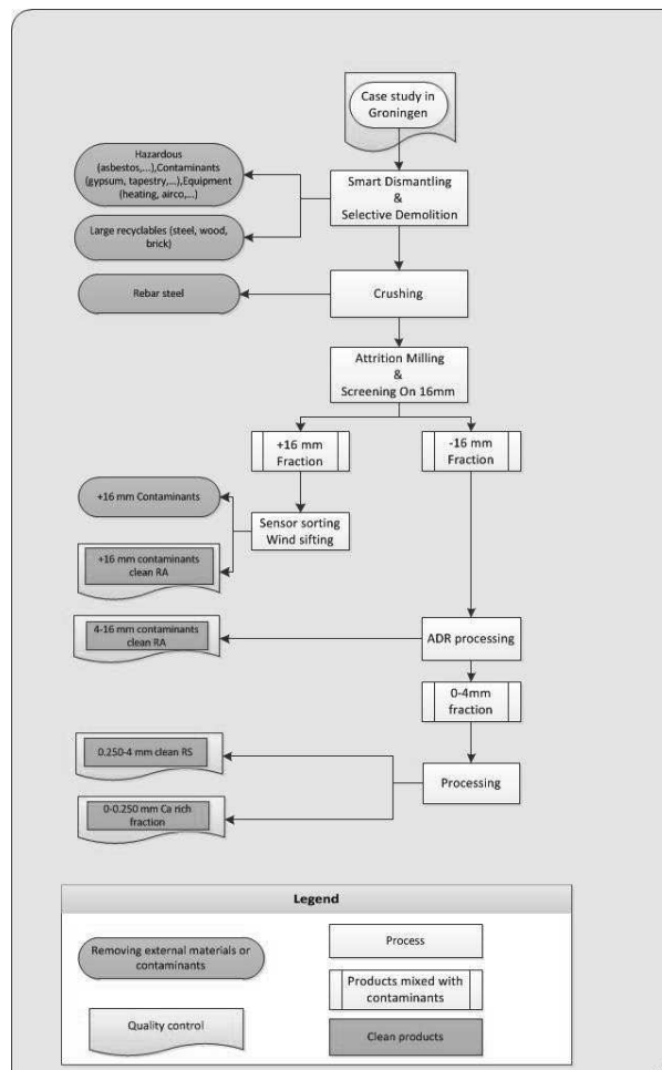
Figure 1: General layout of the C2CA technology showing different steps for contaminants removal. Two developing sensors (HSI and LIBS) are being developed for the quality control of the products.
