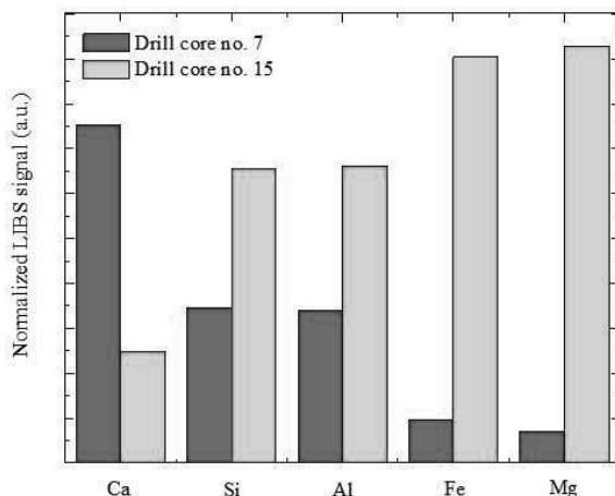
Figure 14: Element-wise comparison of drill cores 7 and 15. Note that the y-axis adds up to unity for each element.
