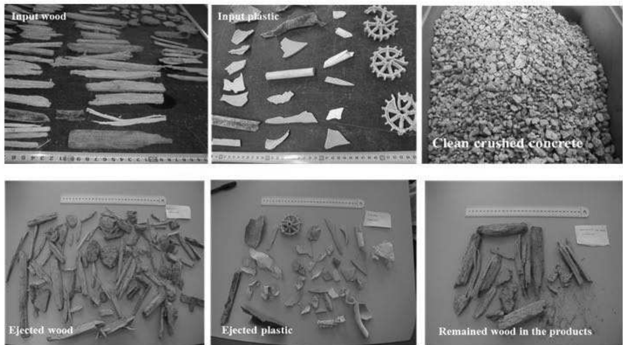
Figure 11: Input of wind sifter (upper images) which consists of wood, plastic and clean +16 mm crushed concrete. Downer images demonstrate the removed wood and plastic using wind sifter and remained wood in the products.
