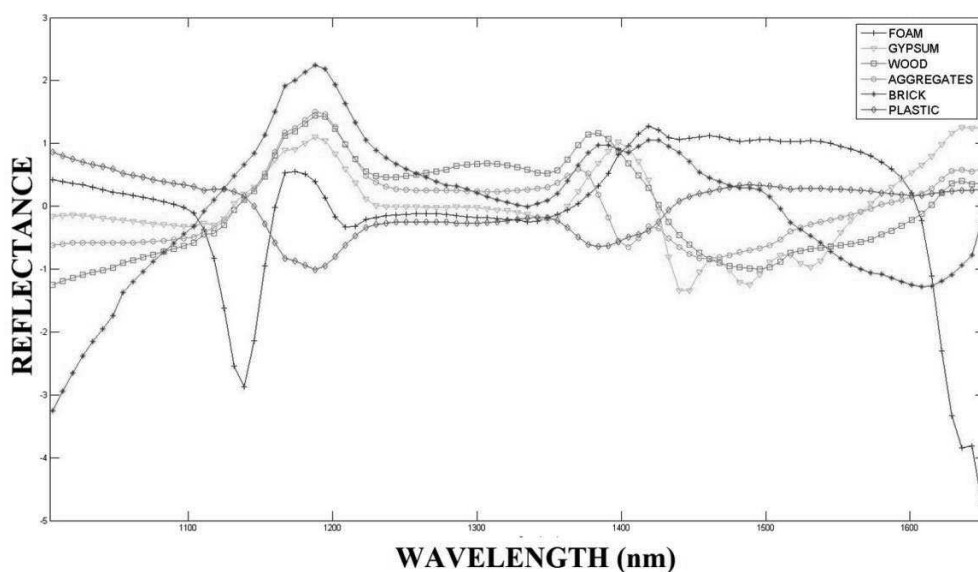
Figure 18: Pre-processed spectra of the six different analysed materials.
