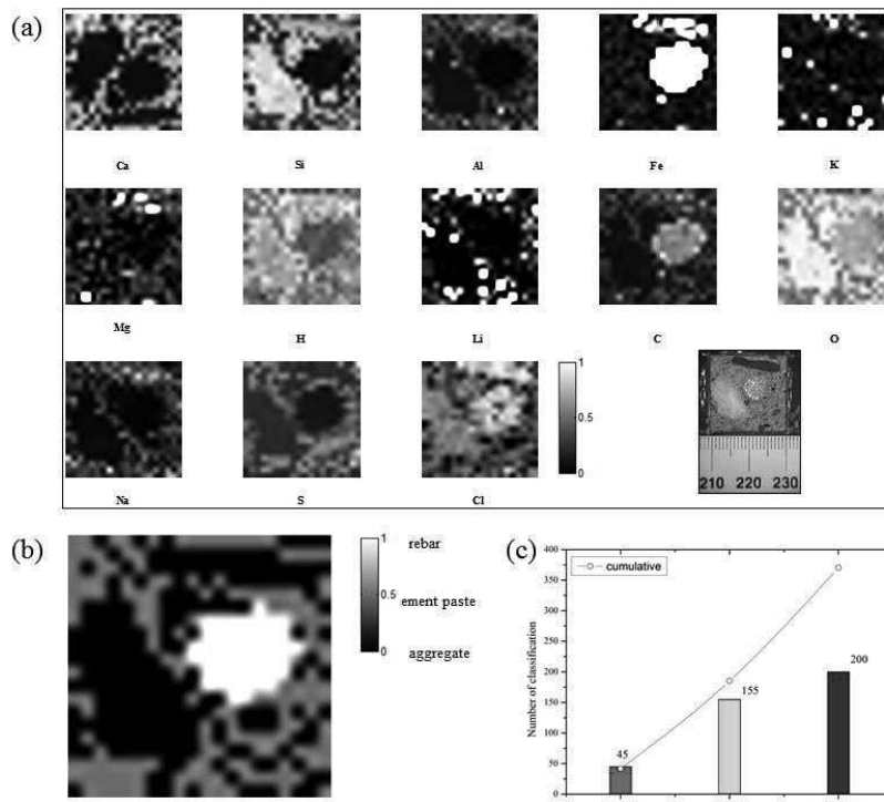
Figure 13: LIBS grid scanning 20 \times 20 \text{ mm}^2 on drill core no. 7 in 1 mm steps. The laser spot diameter is 300 \mu\text{m} . (a) 2D distribution of Ca, Si, Al, Fe, K, Mg, H, Li, C, O, Na, S and Cl. The data are normalized to unity, corresponding to white in a grey scale. (b) classification of rebar, cement paste and aggregate/sand using PCA-neural network algorithm, corresponding to 1, 0.5 and 0 in the grey colour bar, respectively; (c) cumulative number of shots for each material, indicating the area ratios.
