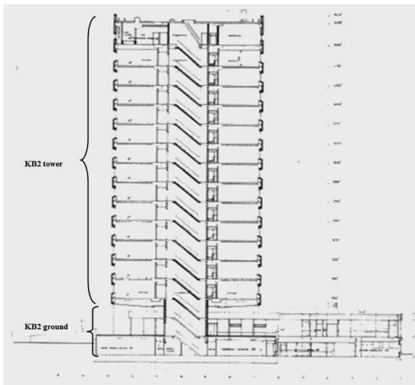
Figure 3: Section plan of the EOL building
