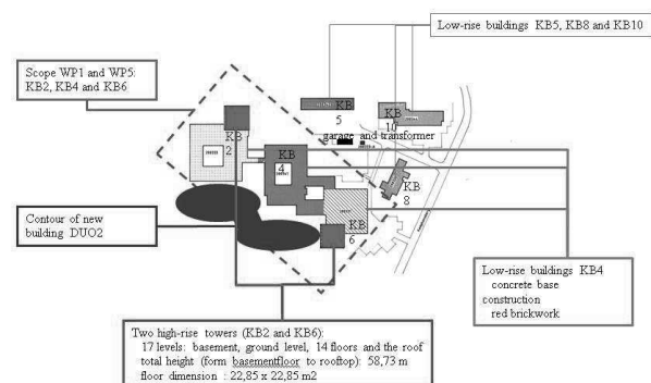
Figure 2: Overview of the end of life buildings
