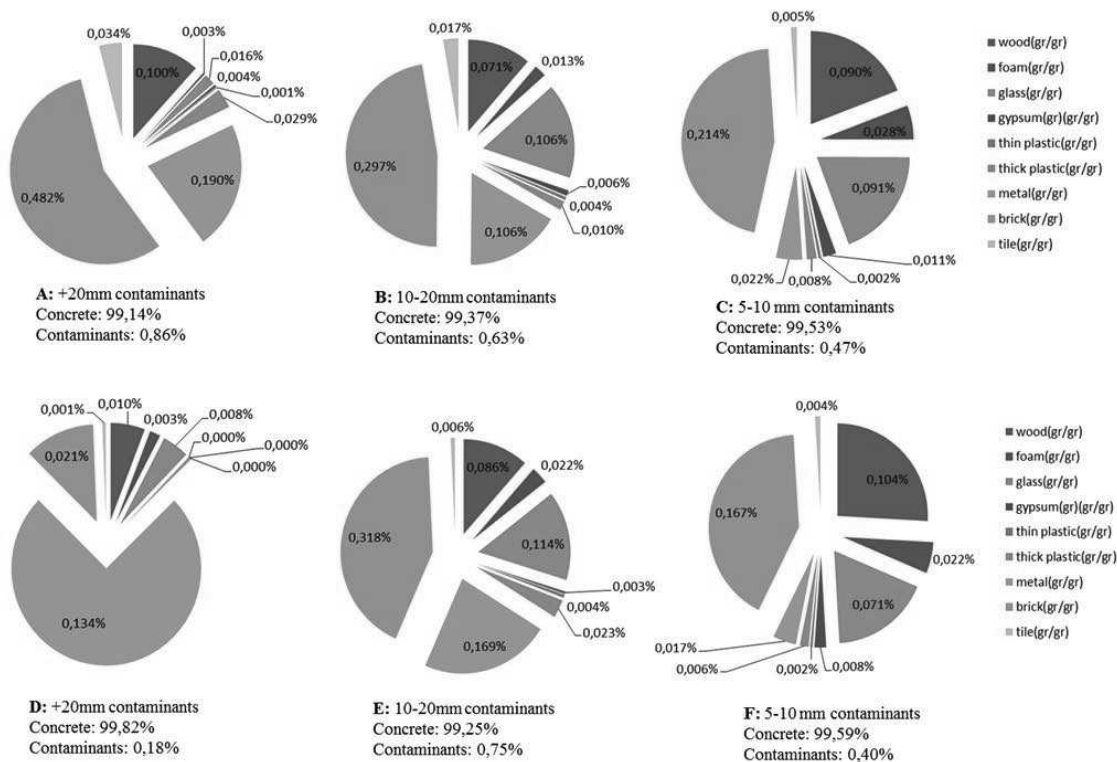
Figure 6: A, B and C show the amount of contaminants in the +5mm input of the autogenous mill. D, E and F show the amount of contaminants in the +5mm output of the autogenous mill.
