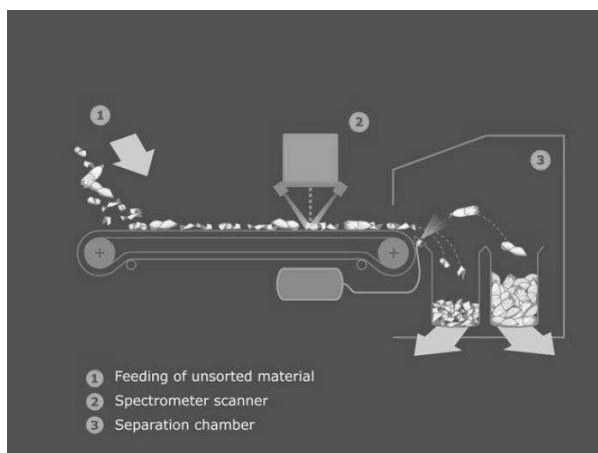
Figure 8: Functional principle of TOMRA NIR sensor sorting technology.
