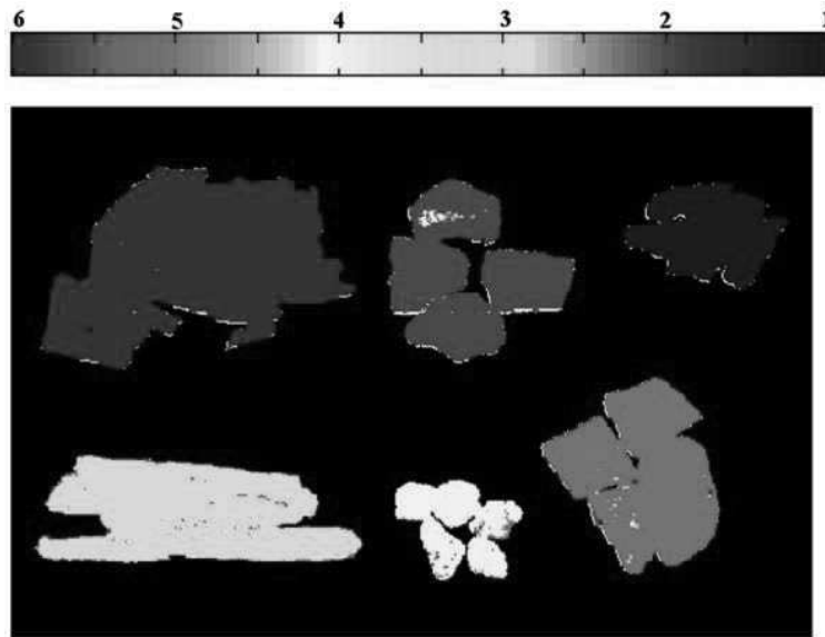
Figure 20: Prediction map based on PLS-DA model built for the classification of foam (1), gypsum (2), wood (3), aggregates (4), brick (5) and plastic (6) in the Experimental set up 2.
