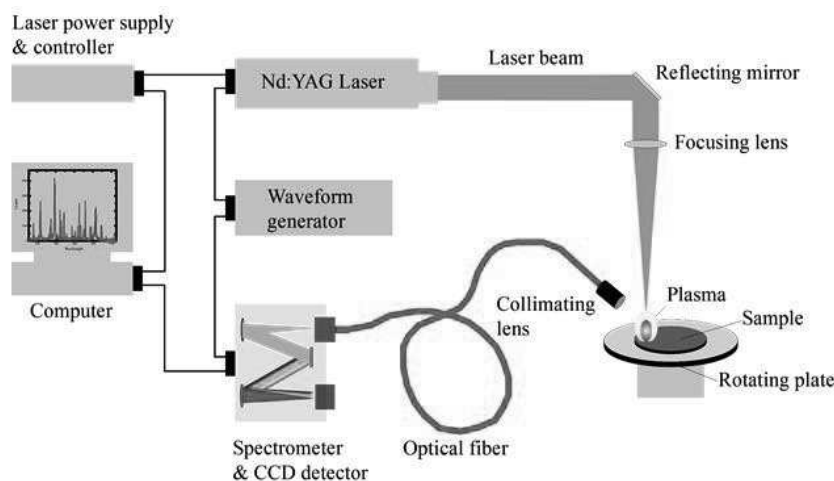
Figure 12: Laboratory LIBS experimental setup.
