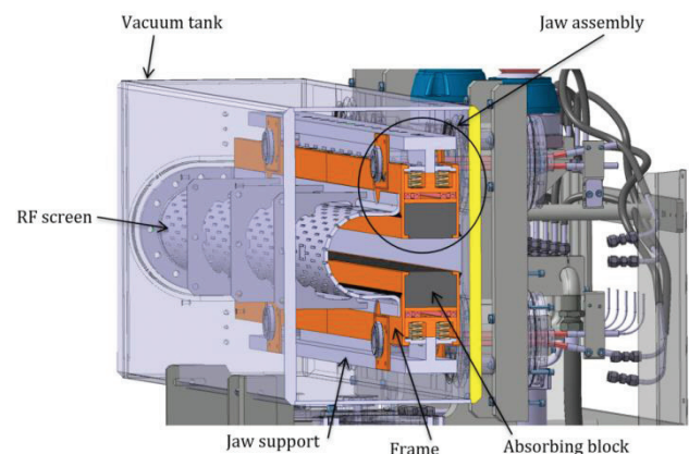
Figure 1: Preliminary design of one TDIS module.
