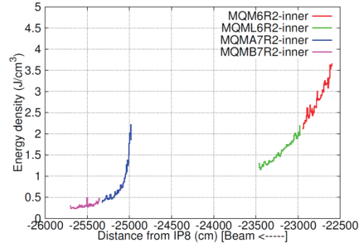
Figure 5: Longitudinal peak energy density in the inner coils of the quadrupoles Q6 and Q7.
