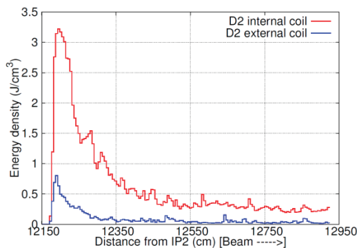
Figure 4: Longitudinal peak energy density in D2 coils.
