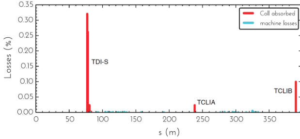
Figure 3: Simulated loss map of Beam 1 in case of MKI kick error of \sim 11\% (grazing impact on TDI in case of ideal machine) considering the machine configuration where the highest losses were seen on the TCLIB.
