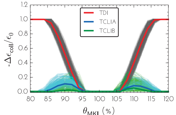
Figure 2: Single particle 5\sigma emittance cut at the three injection protection devices as function of MKI kick for 500 different machine configurations. The solid thick lines represent the average value for the different machine configurations.
