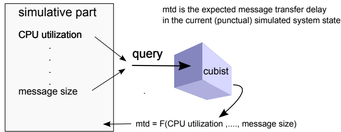
Figure 6: Coupling of simulative and machine learning components.
