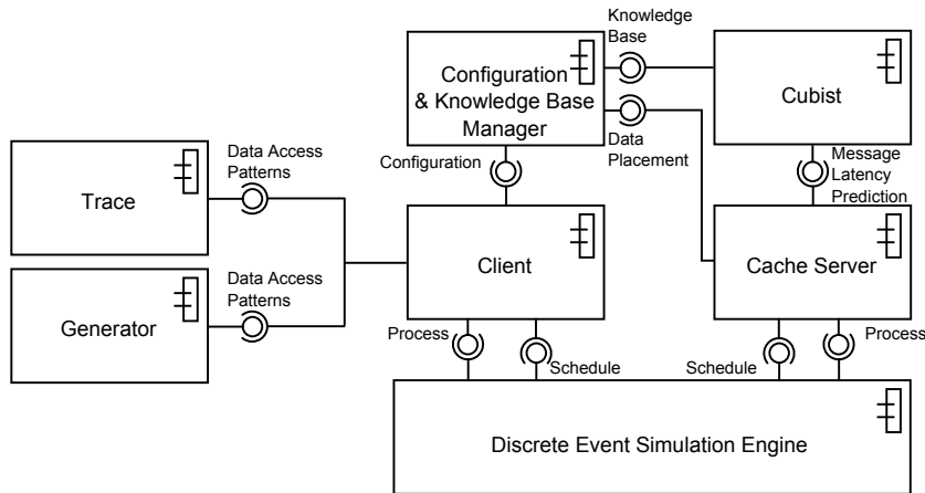
Figure 7: Components diagram.
