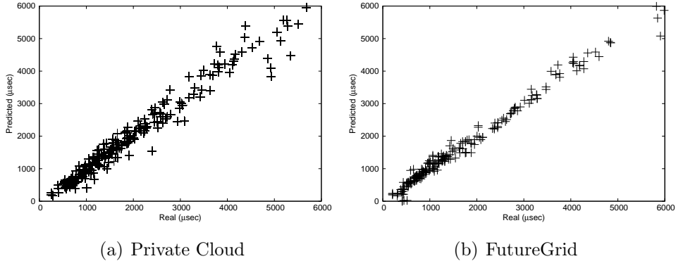
Figure 16: Scatter plot evaluating the 10-fold cross-validation accuracy of the Cubist models that predict the message delivery latency.
