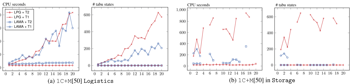
Fig. 8. CPU time and number of generated tabu states of RealizePlanProg using LPG and LAMA with/out achieving the next maintenance goals for planning programs with domains Logistics and Storage and \delta equal to 1C+M[50]. The x-axis refers to the program number (the greater the number is, the greater the size of the planning domain is). The legend from the first chart applies in all four charts.
