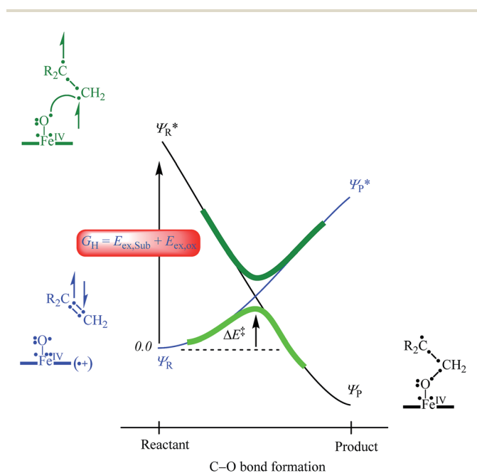
Fig. 8 VB curve crossing diagram for the C–O bond formation step in olefin epoxidation ( \text{R}_2\text{C}=\text{CH}_2 ) by [\text{Fe}^{\text{IV}}(\text{O})(\text{TPFP}^{\bullet+})]^+ . Valence electrons are identified with a dot and lines (curved and straight) in the VB structures represent bonds.
