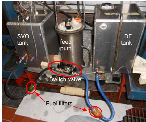
Figure 2. Bi-fuel system.
