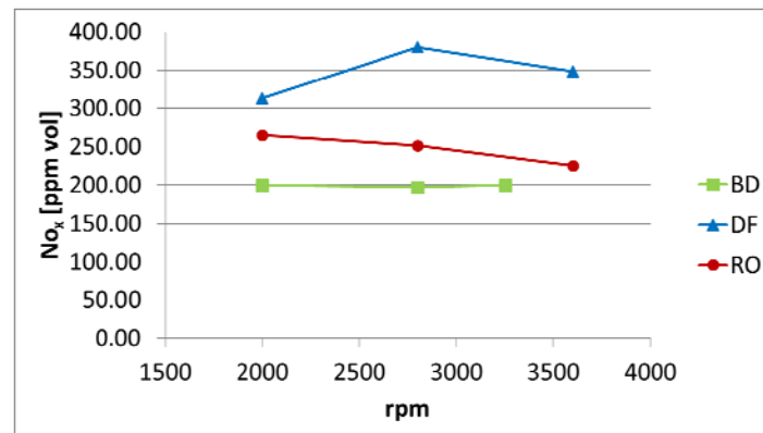
Figure 8. NO x concentration in exhaust.
