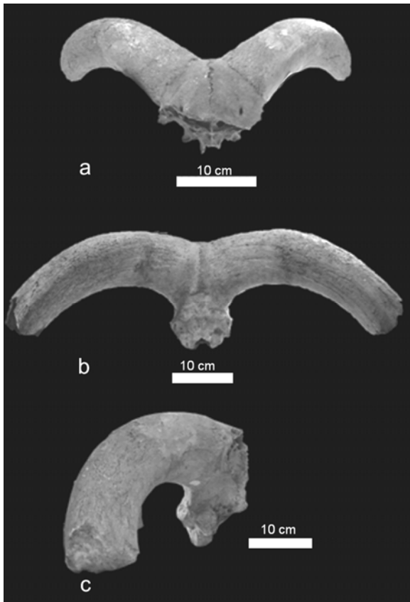
Fig. 2 - Incomplete skull of Ovis ammon antiqua from the Magliana area; a) frontal view; b) posterior view; c) lateral view.
