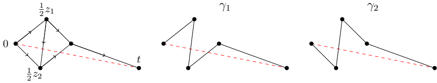
Fig. 4 Sketch of the construction used in the upper bound of Lemma 4.5. The left panel shows the support of the measure, the central one the part on which \alpha_1 \neq 0 , the right one the part on which \alpha_2 \neq 0 . The red dashed line is t
