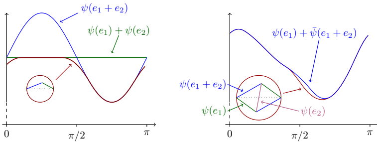
Fig. 5 Left panel \bar{\psi}(e_1 + e_2, t) as given in Lemma 4.6 as a function of \alpha , for \eta = 1, t = (\cos \alpha, \sin \alpha) . The two one-dimensional options \psi(e_1, t) + \psi(e_2, t) = 2 + \eta and \psi(e_1 + e_2, t) = 2 + \eta(1 + 2t_1 t_2) are optimal for different orientations. Close to the intersection a mixture of the two options is optimal, as sketched in the inset. Right panel corresponding plot for \bar{\psi}(2e_1 + e_2, t) (different vertical scale). For most values of t the optimal energy is obtained using \psi(e_1, t) + \bar{\psi}(e_1 + e_2, t) . The latter is the convex, subadditive envelope of \psi , see discussion at the end of Sect. 4.3. However, there is a region in which a more complex structure develops (sketched in the inset), leading to a lower energy. The latter construction bears similarity to the examples given in [2,4]
