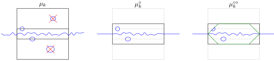
Fig. 3 Passing from \mu_k to \mu_k^{\circ} . The squares represent R_{1,1}^t , the rectangles R_{1,h}^t and R_{1,2h}^t
