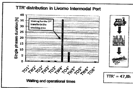
Figure 24: Model application results – Livorno Port (unit entering on train, exiting on ship).
