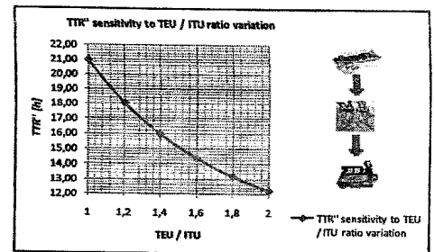
Figure 27: TTR'' sensitivity analysis to the TEU / ITU ratio variation.
