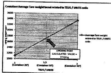
Figure 22: Determination of mean unit tare weight
