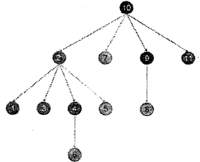
Figure 14: Shortest path starting from TEU (threshold R=0.8 )
