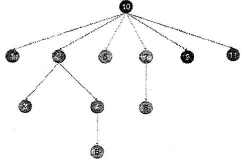
Figure 13: Shortest path starting from TEU (threshold R=0.7 )
