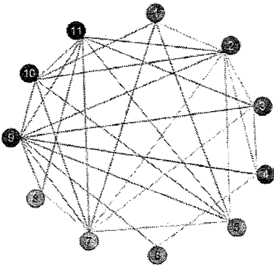
Figure 10: graph of the relevant correlations with R > 0.7
