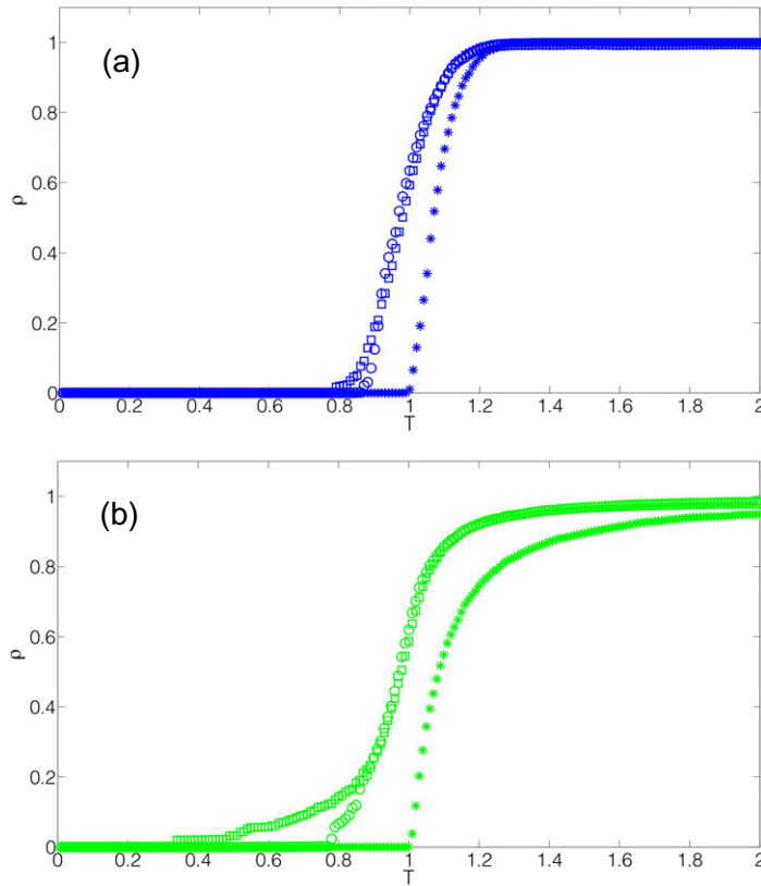
Figure 6. (a) Comparison of the resistivity curves for a Gaussian T_c distribution ( \mu = 1 , \sigma = 0.1 ) in a uniform system (stars), in an SRW cluster (circles) and in a DLA cluster (squares). (b) Comparison of the resistivity curves for a Cauchy T_c distribution ( \mu = 1 , \gamma = 0.08 ) in a uniform system (stars), in an SRW cluster (circles) and in a DLA cluster (squares).
