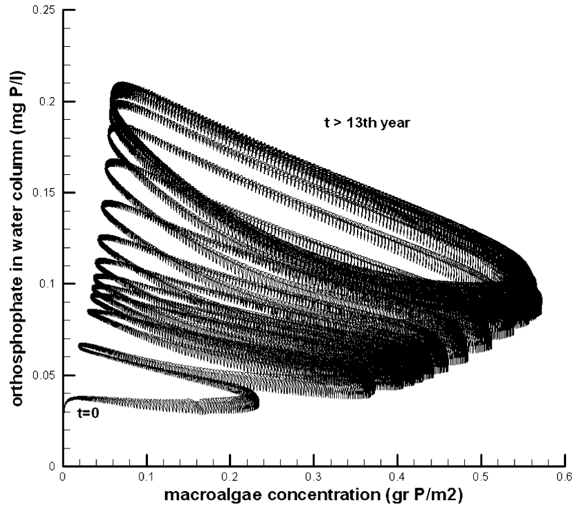
Fig. 5. – Phase plane orthophosphate vs. macroalgae ( q_{\text{poiimm}} = 5 \times 10^{-8} \text{ g/m}^3 ).
