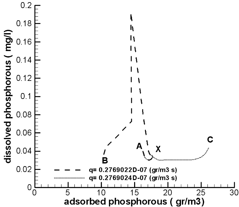
Fig. 9. – Poincarè section: dissolved vs. adsorbed phosphorous.
