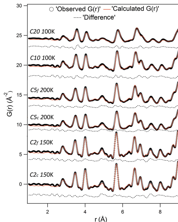
Figure 3 Example of local structural fits performed between 1 and 10 Å as a function of composition and particle size.
