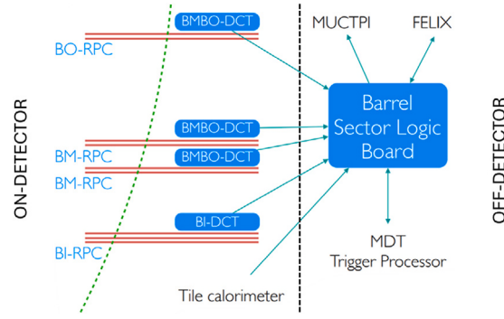
Fig. 1. Simplified schema of the L0 Muon Barrel Trigger System.
