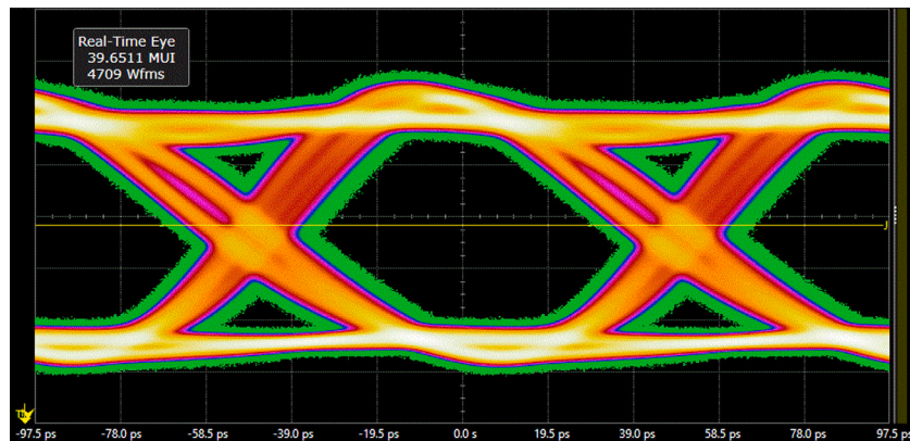
Fig. 2. Uplink Eye diagram.
