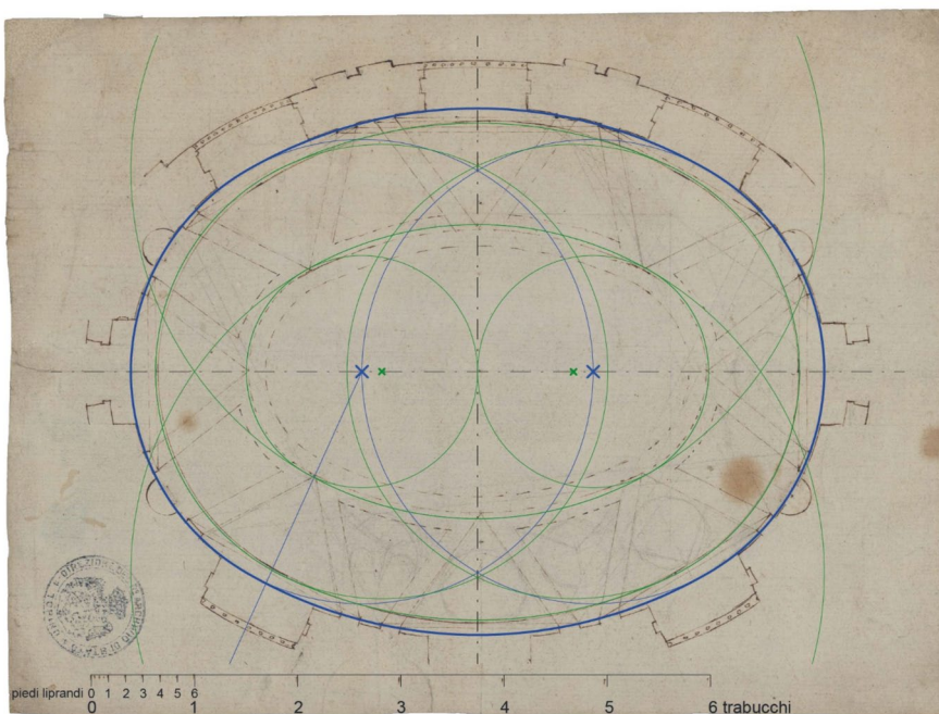
Fig. 7 Palazzo Carignano, design drawing of the main hall at the noble plan. Superimposition of the geometric construction following Millon (1970). In blue: geometric construction of the oval with the major axis equal to three radii of the circumference that shapes the interior perimeter of the main hall. In green: the other constructions by Millon for defining the central oval of the dome. Image: Archivio di Stato di Torino – Sezioni Riunite, Disegni Azienda Savoia—Carignano Torino Palazzo Carignano, Cat. 53, m. 1, fasc. 9, n. 9. Digital redrawing: Roberta Spallone (color figure online)
