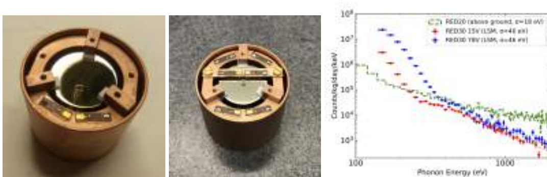
Figure 3: Left and center panels: picture of the 33.4 g EDELWEISS detectors RED20 and RED30, respectively, in their copper holder. The exposed side shows the Ge-NTD thermistances glued on the top side. Right : Efficiency-corrected event rates, in events per kgd and per keV, as a function of the total phonon energy in eV. Green dashed: RED20. Red and blue points: spectra recorded by RED30 with biases of 15 and 78 Volt, respectively. The rises below 300 eV correspond to the onset of the read-out noise. The lines are fits to guide the eyes.
