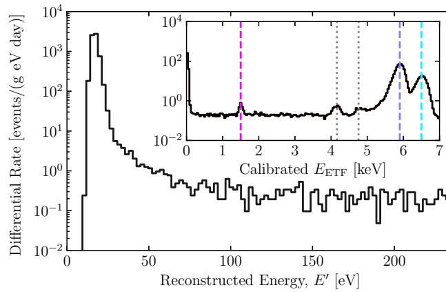
Figure 12: Measured energy spectrum in the DM-search ROI for the full exposure after application of the quality cuts. The data have been normalized to events per gram per day per eV and have been corrected for the event-selection efficiency, but not the trigger efficiency. The inset shows the calibrated E_{\text{ETF}} spectrum up to 7 keV, noting the locations of the different spectral peaks. The known values of the dashed lines are 1.5, 5.9, and 6.5 keV for the Al fluorescence (pink), ^{55}\text{Fe} K_\alpha (blue), and ^{55}\text{Fe} K_\beta (cyan) lines, respectively. The two dotted gray lines between 4 and 5 keV in calibrated E_{\text{ETF}} are the Si escape peaks [56]. Figure and caption from Ref. [13].
