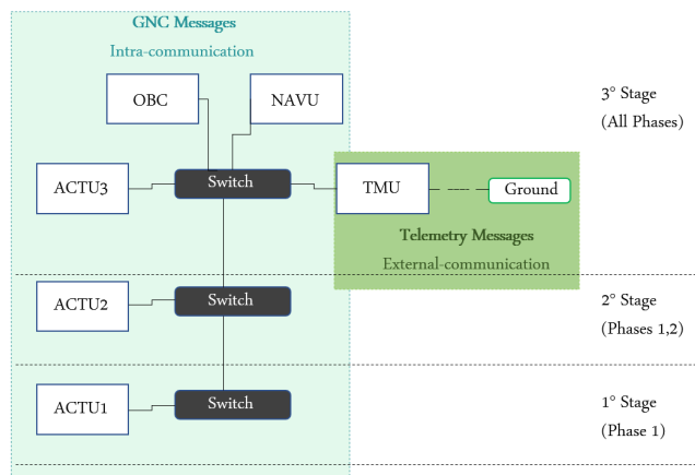
FIGURE 11. Network topology.
