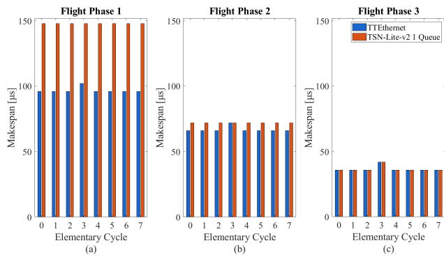
FIGURE 14. Makespan values comparison for TT Ethernet and TSN-Lite-v2 as a function of the EC index in the Flight Phases 1 (a), 2 (b) and 3 (c). TSN-Lite-v2 case with one queue available per egress port.
