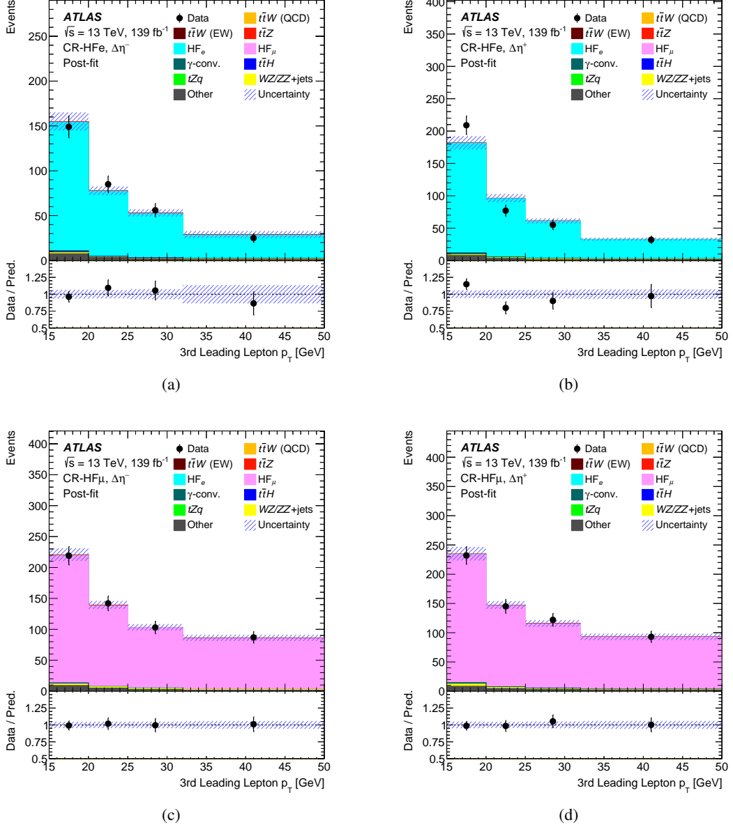
Figure 3: Comparison between data and the post-fit predictions in (a,b) CR-HF e and (c,d) CR-HF \mu . The distributions show the p_T of the third lepton (electron or muon), which is the variable that is used for the binned likelihood fit. The regions are separated between \Delta\eta_{\text{BDT}}^\ell \leq 0 ( \Delta\eta^- ) and \Delta\eta_{\text{BDT}}^\ell > 0 ( \Delta\eta^+ ). The error bands include the total uncertainties in the post-fit predictions, with the exception of the \Delta\eta^\pm CR-dependency uncertainty. The ratios of the data to the total post-fit predictions are shown in the lower panels. Events with the p_T of the third lepton above 50 GeV are included in the rightmost bins.
