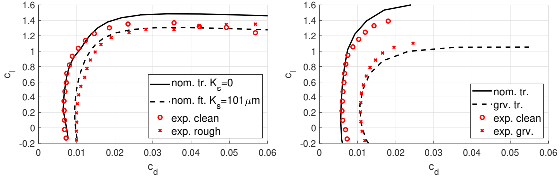
Figure 3: Comparison of CFD vs. experiments for a NACA63 418 with distributed roughness of K_s = 101 \mu\text{m} (left) and 3 mm LE groove (right).
