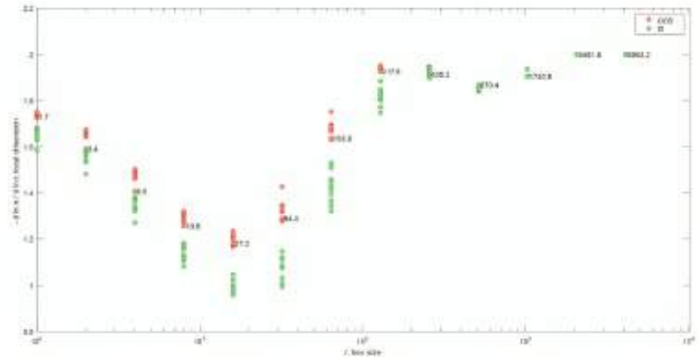
Figure 16. Local fractal dimension as a function of the computation box size for the sample condition. The corresponding computation box sizes in \mu\text{m} are indicated at the local fractal dimension values.
