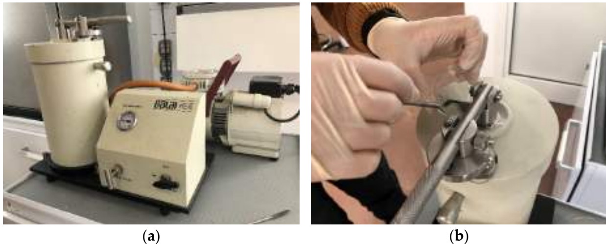
Figure 2. GALAI PD-10 vacuum gauge (a) and sample dispersion on the device's chamber (b).
