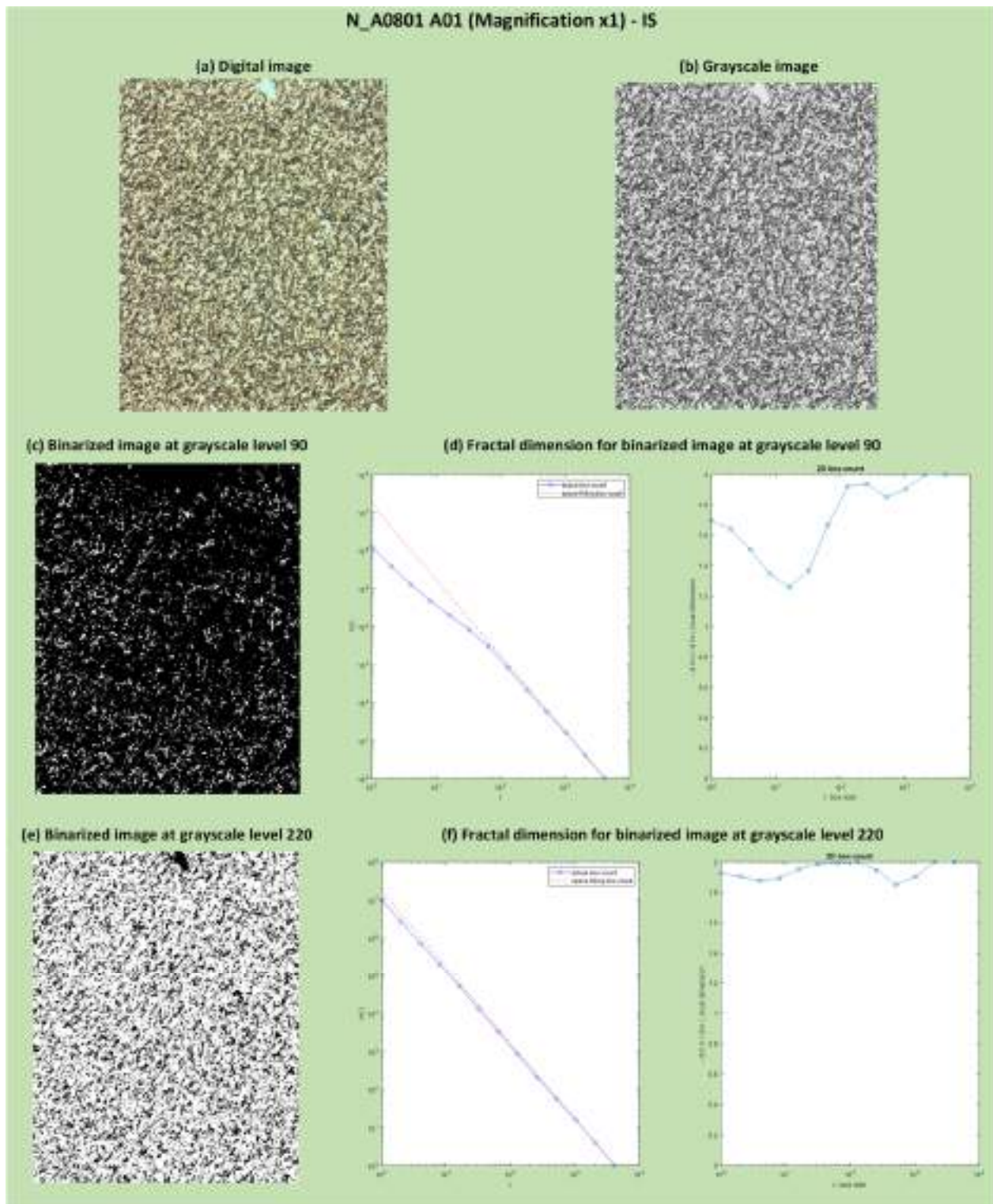
Figure 12. Results of binarization at grayscale levels 90 and 220 and calculation of fractal dimension on the binarized images: IS sample (N_A0801 A01 at Magnification \times 1 ): digital image (a), grayscale image (b), binarized image at grayscale level 90 (c), fractal dimension for binarized image at grayscale level 90 (d), binarized image at grayscale level 220 (e) and fractal dimension for binarized image at grayscale level 220 (f). In (d,f), the local fractal dimension as a function of box size and the number of boxes as a function of box size are shown. The red dashed line represents the space-filling curve, which fills a 2D unit box to map the powder sample in the plot. The blue line, the actual box count, aligns the space-filling curve with the scaling exponents measured by the algorithm.
