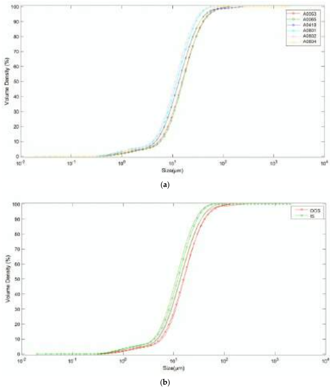
Figure 4. Particle size distribution of the samples labeled according to sample ID (a) and product requirement compliance (i.e., ‘Out of Specification’, OOS, or ‘In Specification’, IS, categories) (b). The samples labeled A0065, A0418, and A0053 correspond to the OOS category, while A0801, A082, and A0804 correspond to the IS category. Particle size distributions (PSDs) were obtained by laser diffraction. At the same particle size, the IS samples generally exhibit a lower volume density compared to the OOS samples. PSD curves of the OOS samples are slightly shifted to the right (or skewed) compared to the PSD curves of the IS samples.
