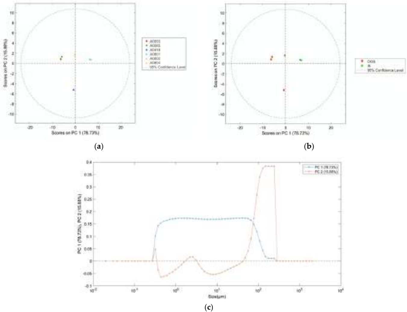
Figure 5. PCA scores plot (PC1 vs. PC2) of the particle size distribution for samples (a) and conditions (b) and PCA loadings plot (c). The 95% confidence level reported in the PCA scores plot represents the statistical certainty regarding the dispersion of data points around their respective centroids or means.
