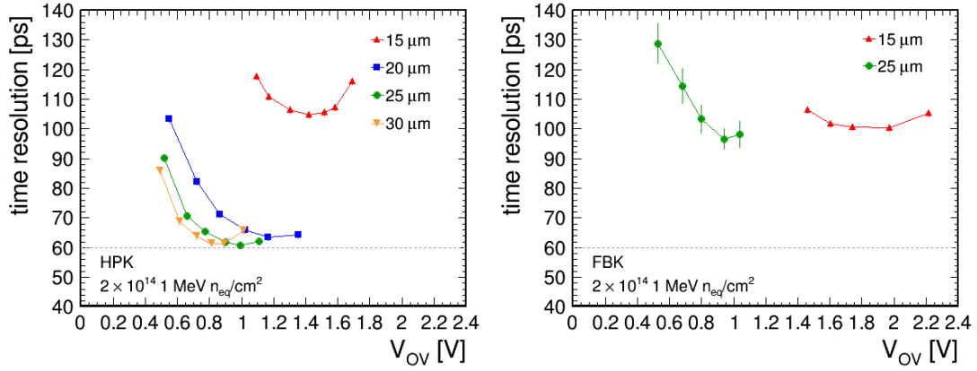
Figure 8. Time resolution as a function of the SiPM over-voltage for modules with SiPMs of different cell-sizes irradiated to 2 \times 10^{14} \text{ n}_{eq}/\text{cm}^2 . All measurements were taken at an operational temperature of -35^\circ\text{C} . Left: modules with SiPMs from HPK. Right: modules with SiPMs from FBK.
