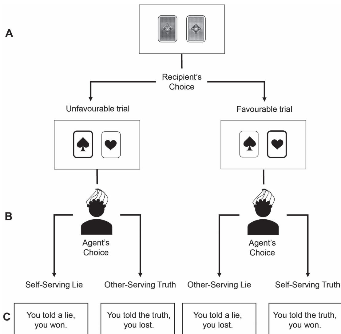
Fig. 1. Illustration of task structure. A) The recipient (opponent) makes a blind choice between 2 down-facing cards. B) The agent (participant) shown here with electrodes can see the initial outcome and can either choose to tell the truth or lie to the recipient. The final outcome of the trial depends on the agent's decision. C) Immediately, after their response, the agent received feedback pertaining to the outcome of the trial.
