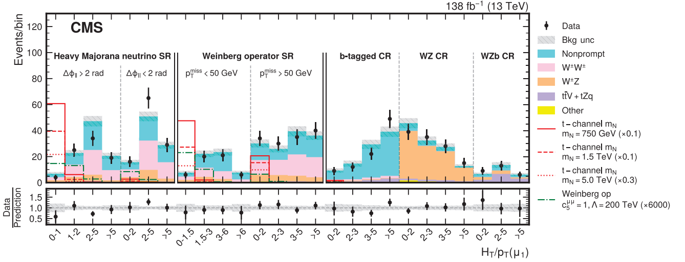
FIG. 2. The H_T/p_T^{\mu_1} distribution in the SRs and CRs. The horizontal axis indicates the bin width. The predicted yields of the backgrounds are shown with their best fit normalizations from the simultaneous fits for the background-only hypothesis. The lines indicate the scaled expected distributions of the heavy Majorana neutrino process with m_N = 750 GeV (solid red line), 1.5 TeV (dashed red line), 5.0 TeV (dotted red line), and of the Weinberg operator process (dash-dotted green line). The heavy Majorana neutrino processes are characterized by the azimuthal separation variable \Delta\phi_{\ell\ell} , while the Weinberg operator process features in low missing transverse momentum.
