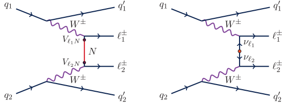
FIG. 1. Example Feynman diagrams of VBF processes with heavy Majorana neutrino production (left) and processes mediated by the Weinberg operator (right) at the LHC.
