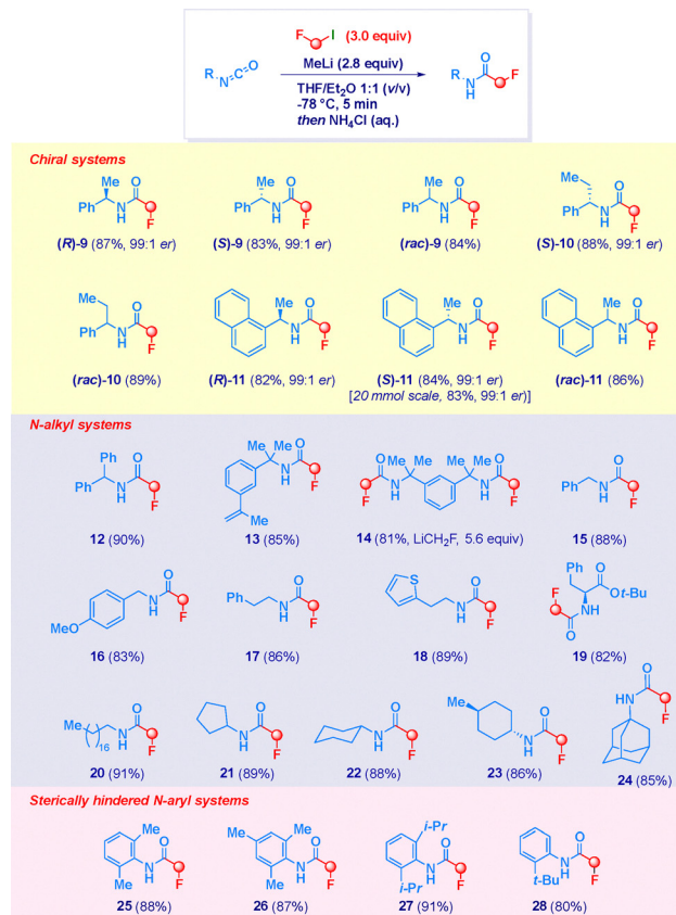
Scheme 3 Scope of the reaction.
