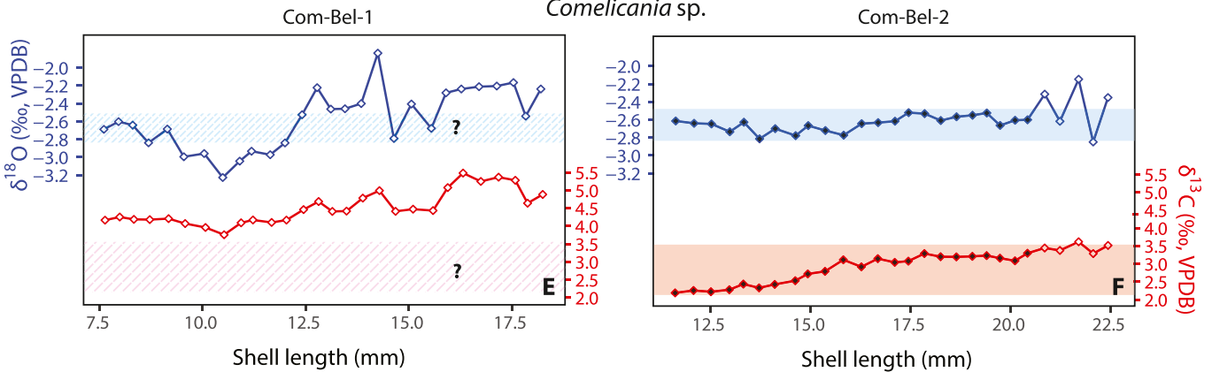
Fig. 6. Intra-generic comparison of profiles of the \delta^{18}\text{O} (blue color) and \delta^{13}\text{C} (red color) along the mid-shell longitudinal section for the different specimens; open diamonds represent samples deemed to be altered based on the screening test; the shadow blue and red areas represent the range of overlap between specimens collected at the same localities; for the Dolomites samples, the shadow areas represent the range of the preserved specimen Com-Bel-1. The direction of shell growth is from left to right in each panel. (For interpretation of the references to color in this figure legend, the reader is referred to the web version of this article.)
