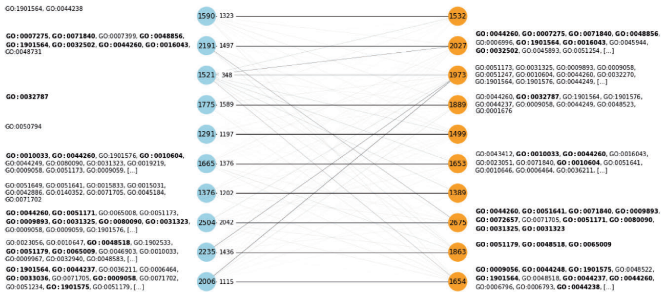
Fig. 3. Cluster analysis on the real and synthetic expression datasets. We performed k -means clustering with k=10 clusters both on the test (real) and the generated datasets. Blue and orange nodes represent real and synthetic clusters, respectively. The value of each node corresponds to the number of genes of that cluster. We matched real and synthetic clusters according to the number of shared genes and, for each real cluster, we display as edge labels the number of matching genes for the top association. The width of each edge is proportional to the number of shared genes. We further performed an overrepresentation test using GOfuncR (Grote, 2020) with a family-wise error rate threshold of 0.05. We show the enriched Gene Ontology terms next to the corresponding cluster and highlight in bold those that are common between each top matching pair of clusters (see Supplementary Appendix SF for a detailed list on the enriched Gene Ontology terms). These results suggest that gene clusters and enriched biological processes are similar at a global scale
