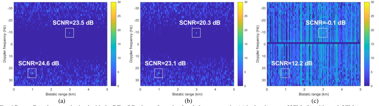
Fig. 4 Range-Doppler map obtained with the RF + SC scheme for a simulated clutter scenario: (a) in the absence of ICM; (b) with weak ICM ( \sigma_v = 0.01 m/s) (c) with strong ICM ( \sigma_v = 0.1 m/s)
