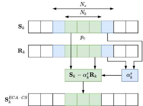
Fig. 5 Sketch of the ECA-CS flow diagram.
