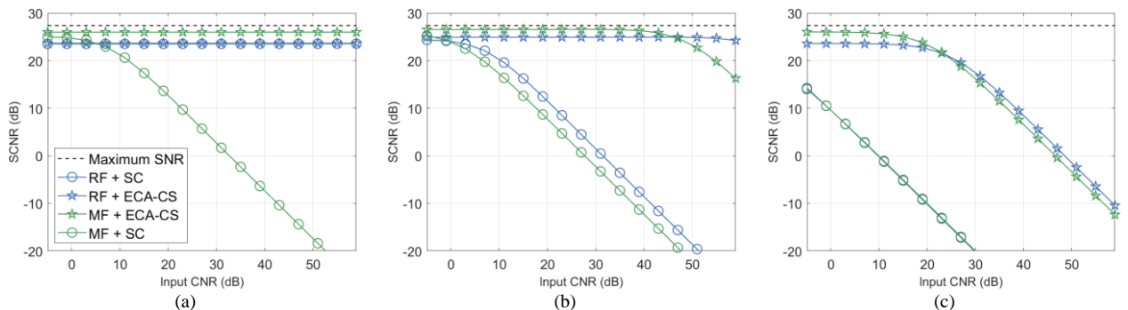
Fig. 9 Achievable SCNR for a point-like target as a function of the input CNR for a simulated clutter scenario: (a) in the absence of ICM; (b) with weak ICM ( \sigma_v = 0.01 m/s) (c) with strong ICM ( \sigma_v = 0.1 m/s).
