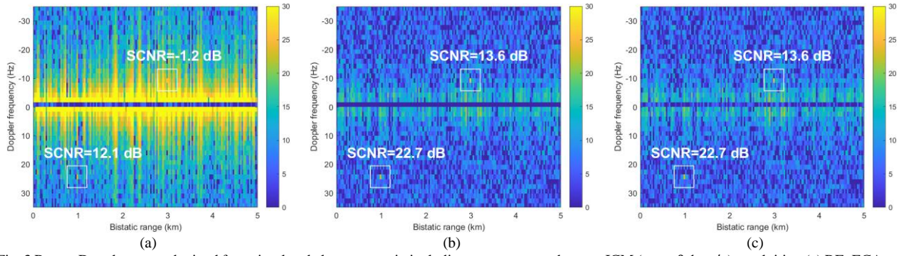
Fig. 3 Range-Doppler maps obtained for a simulated clutter scenario including two targets and strong ICM ( \sigma_v = 0.1 m/s): exploiting (a) RF+ECA-C; (b) RF + ECA-CD; (c) ECA-CD + RF.
