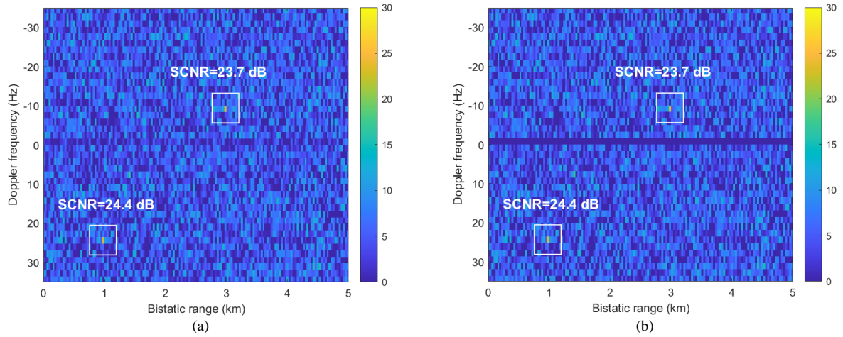
Fig. 2 Range-Doppler maps obtained for a simulated clutter scenario including two targets and no ICM: (a) exploiting the ECA-C + RF scheme; (b) exploiting the RF + ECA-C scheme. A simulated DVB-T signal is assumed as a reference signal.
