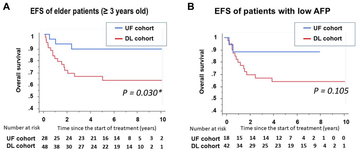
Fig. 4: Event-free survival (EFS) of the upfront (UF) and delayed (DL) surgery patients in the subgroup of over 3 years old at diagnosis and that with low AFP levels. In the patients who were diagnosed at more than 3 years old, 5-years EFS was significantly poor ( P = 0.030 ). In the patients with an AFP level 100–999 ng/mL at diagnosis seemed worse but not significantly ( P = 0.105 ).
