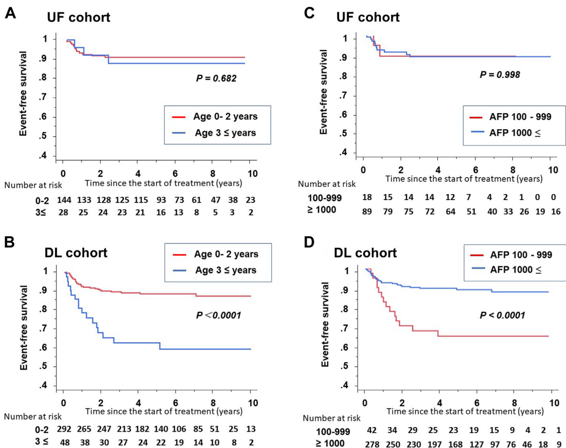
Fig. 3: Event-free survival (EFS) of the upfront (UF) and delayed (DL) surgery patients by age at diagnosis (A and B) and by AFP level at diagnosis (C and D). A. In the UF cohort, 5-year EFS of the patients over 3 years old at diagnosis was slightly worse than other patients, but not significantly. B. In the DL cohort, 5-year EFS of the patients over 3 years old at diagnosis was significantly worse than other patients ( P < 0.0001 ). C. In the UF cohort, 5-year EFS of the patients with an AFP level 100–999 ng/mL at diagnosis was comparable to other patients. D. In the DL cohort, 5-year EFS of the patients with an AFP level 100–999 ng/mL at diagnosis was significantly worse than other patients ( P < 0.0001 ).
