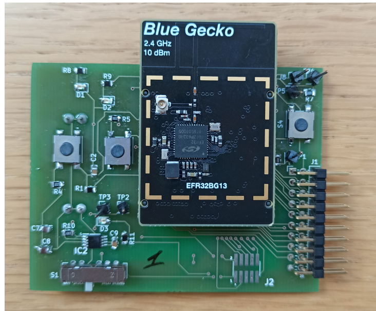
Figure 2. Adopted BLE device with dedicated PCB board.
