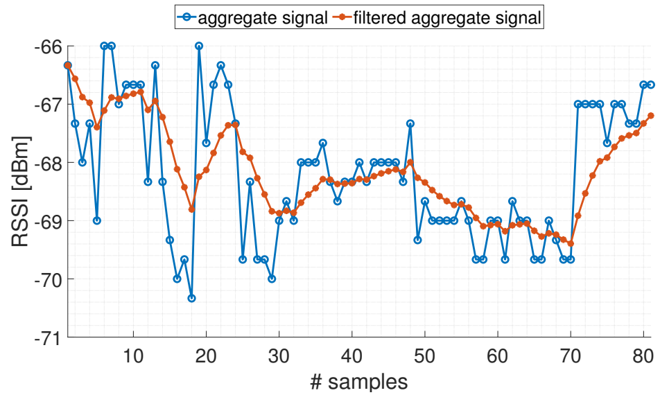
Figure 5. Example of filtering an aggregate signal with mean algorithm.
