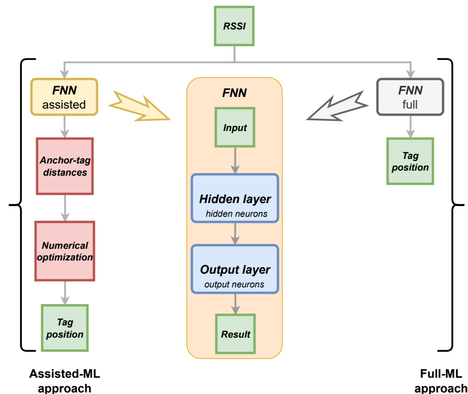
Figure 1. Structure adopted two-layer Feed-Forward Neural Network (FNN) and schematic representations of the Assisted-ML and Full-ML approaches.
