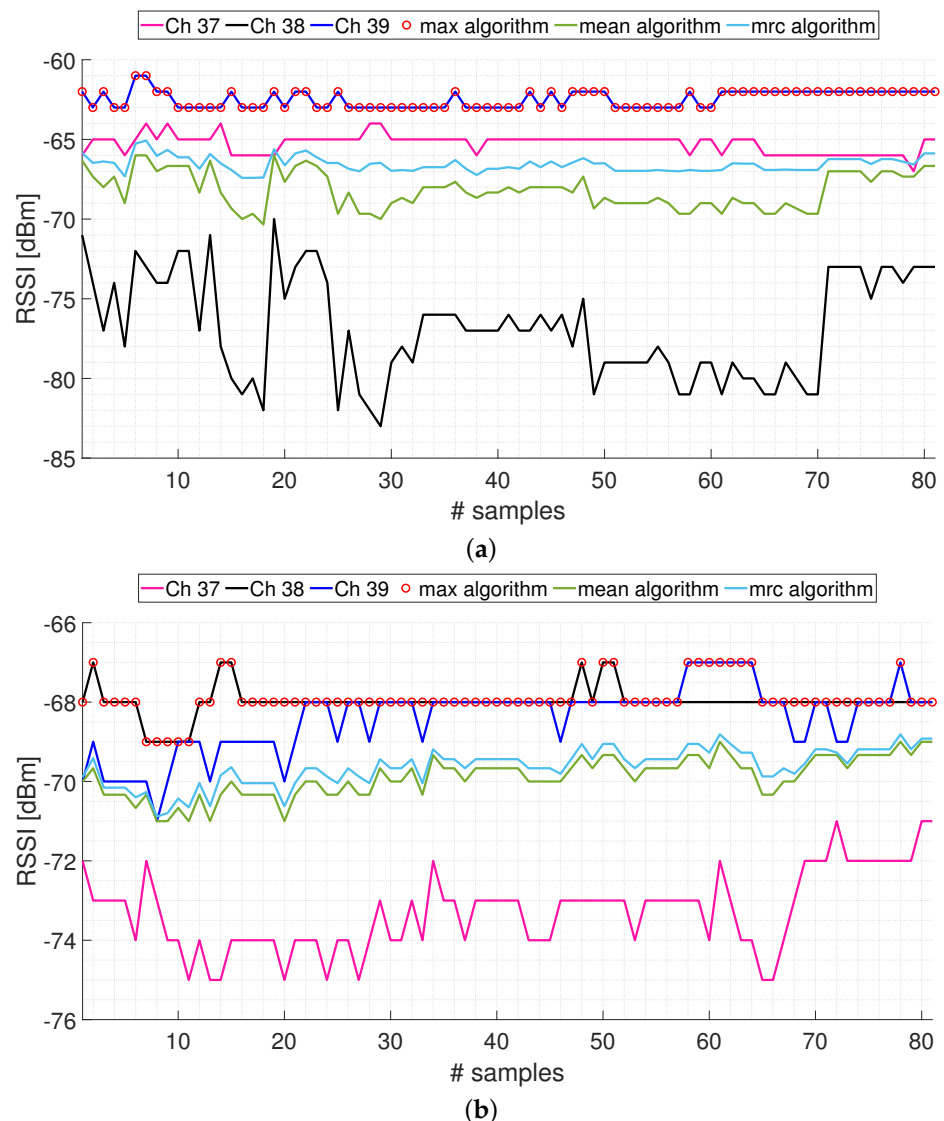
Figure 4. Examples of measured RSSI on the three primary transmission channels (Ch 37, Ch 38, and Ch 39) and adopting the three aggregation techniques (max algorithm, mean algorithm, and mrc algorithm) described in Section 3.1, considering a single anchor-tag pair: (a) anchor-tag distance equal to 2.7 m; (b) anchor-tag distance equal to 5.2 m.
