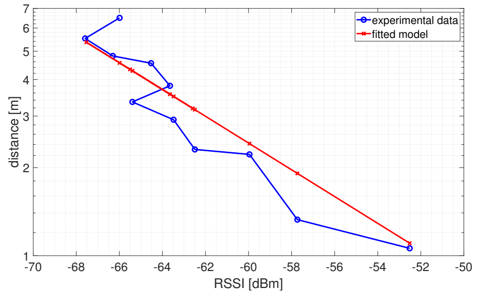
Figure 7. Example of RSSI–distance relationship obtained for anchor A2 and using the RSSI data aggregated with the maximum algorithm and filtered.
