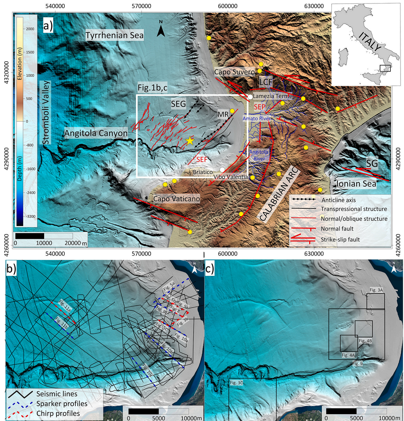
Fig. 1. a) Schematic tectonic sketch map of the S. Eufemia Gulf in the Tyrrhenian Sea (modified from Monaco and Tortorici, 2000 ; Brutto et al., 2016 ) and offshore (modified from Loreto et al., 2013 ; Del Ben et al., 2008 ). Yellow circles indicate M_w > 5 earthquakes from CPTI15 Catalogue ( Rovida et al., 2022 ); the yellow star indicates the location of the 1905 epicentre. LCF: Lamezia-Catanzaro Fault; SEF: S. Eufemia Fault; SEG: S. Eufemia Plain; MR: Maida Ridge. b) High-resolution single-channel seismic track lines collected in the SEG. c) Location of the figures of the bathymetric features shown in the manuscript. (For interpretation of the references to color in this figure legend, the reader is referred to the web version of this article.)
