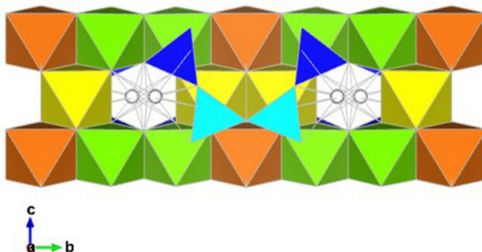
Figure 1. Grunerite structure: projection onto (100) showing the double chain of tetrahedra and the strip of octahedra. Turquoise=T(1), blue =T(2), yellow=M(1), green=M(2), orange=M(3), and white=M(4).
