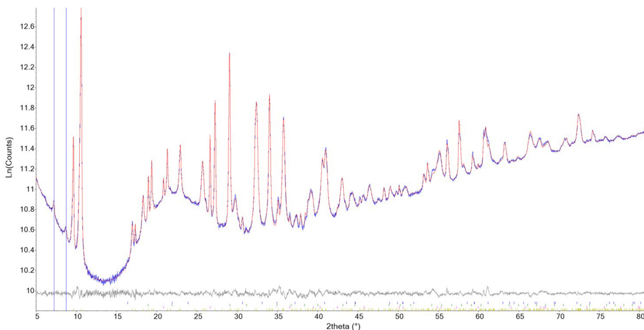
Figure 2. Magnified view (5-80° 2 \theta ) of the Rietveld plots of the refinement of the UICC amosite sample. Intensity scale logarithmic. Blue: experimental; red: calculated; grey: difference; vertical bars indicate the position of the calculated Bragg reflections of (from above to below) ankerite (blue), garnet (green), quartz (magenta) and amosite (yellow). The vertical blue lines indicate the position of the main reflection of stilpnomelane (7.25° 2 \theta ) and biotite/annite (8.45° 2 \theta ), respectively, that were approximated by peaks unrelated to structures.
