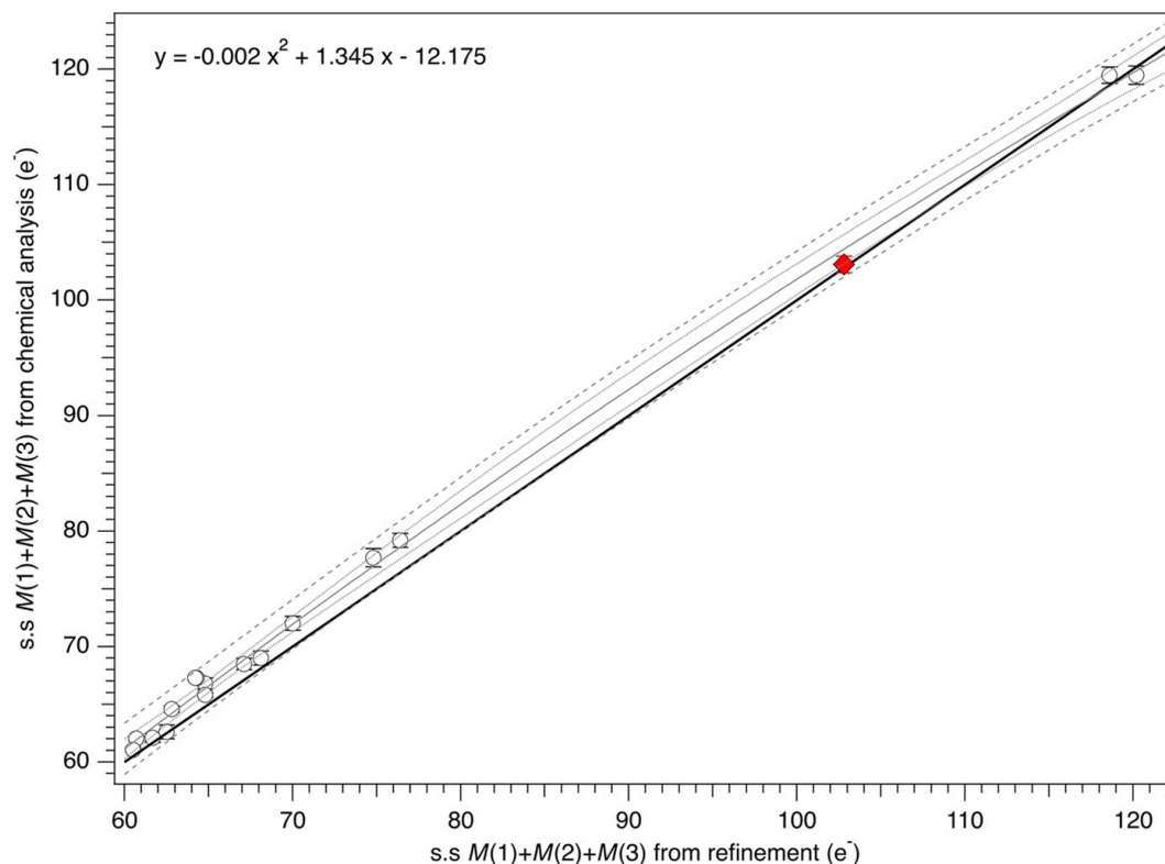
Figure 4. Comparison between the s.s. at C sites obtained by Rietveld refinements performed on data collected in transmission mode and the s.s. at C sites determined by micro-chemical analyses. UICC amosite indicated as a red diamond. Linear regression, confidence (95% level), and prediction intervals are reported as full, short dash, and dotted lines, respectively. Reference data are: Ballirano et al. (2008); Pacella et al. (2008); Andreozzi et al. (2009); Vignaroli et al. (2014); Pacella et al. (2019); Pacella et al. (2021a); Ballirano et al. (2021).
