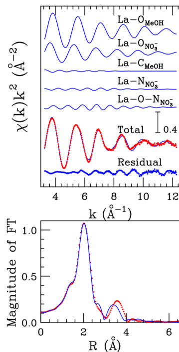
Figure 7. Upper panel: best-fit results for the La K-edge EXAFS spectrum of the 0.1 M \text{La}(\text{NO}_3)_3 methanol solution. From the top the \text{La}\text{--O}_{\text{MeOH}} , \text{La}\text{--O}_{\text{NO}_3^-} , \text{La}\text{--C}_{\text{MeOH}} , \text{La}\text{--N}_{\text{NO}_3^-} , and \text{La}\text{--O}\text{--N}_{\text{NO}_3^-} theoretical signals are shown, together with the total theoretical contribution (blue line) compared to the experimental spectrum (red dots), and the resulting residual (blue dots). Lower panel: nonphase shift corrected FTs of the EXAFS theoretical signals (blue line) and of the experimental data (red dots).
